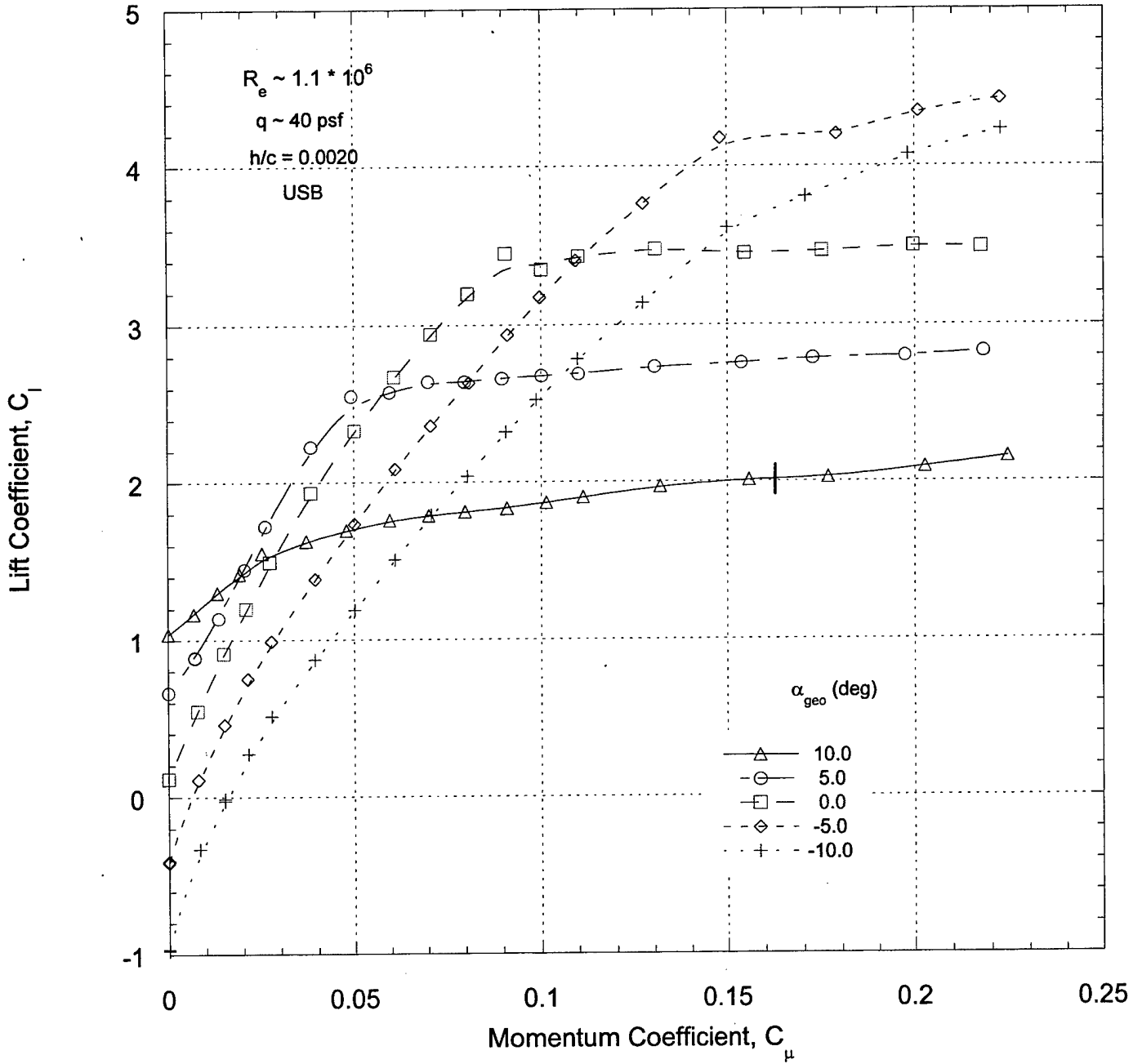
Figure 6a. USB, h/c = 0.0020 .
