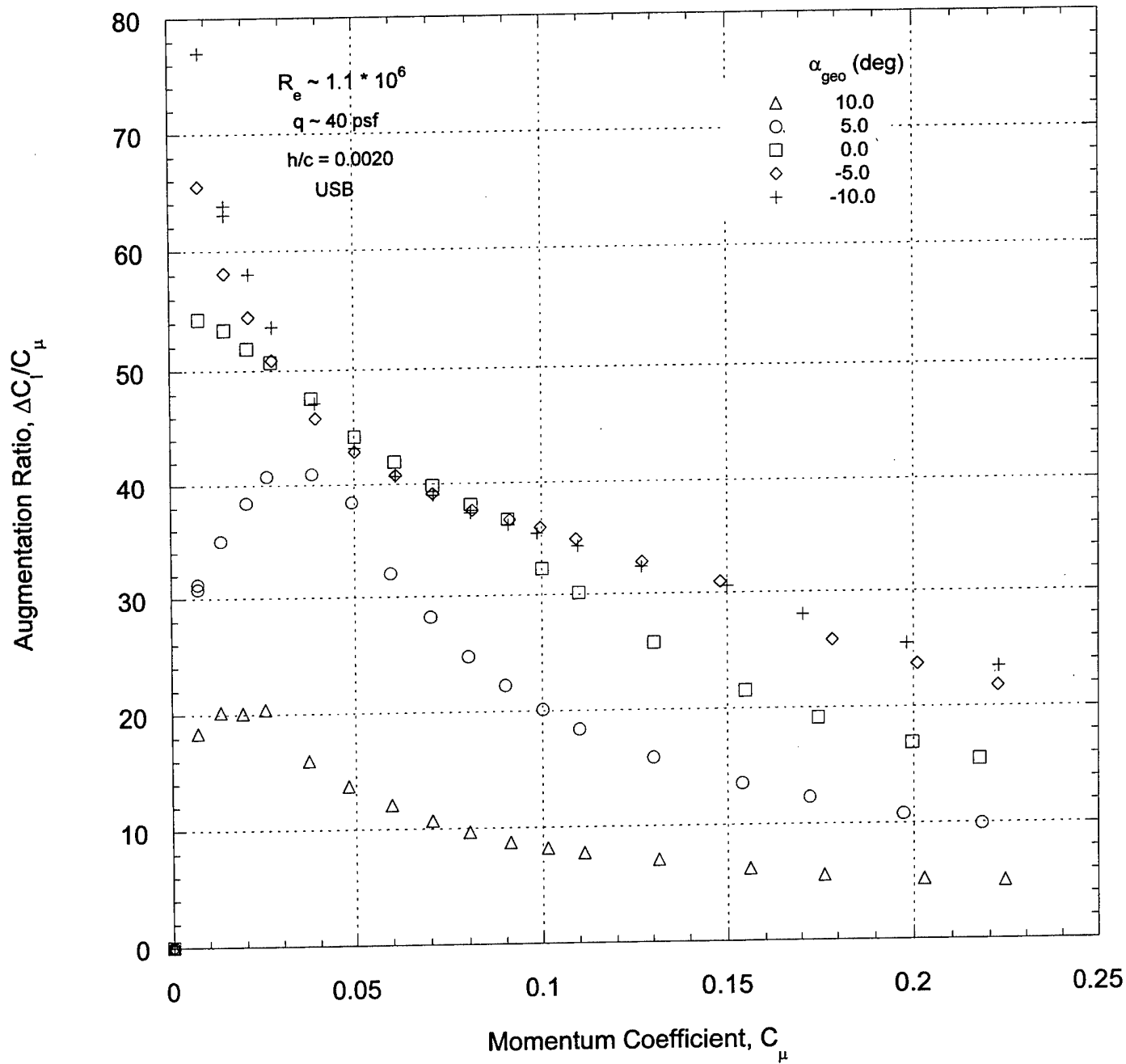
Figure 15a. USB, h/c = 0.0020
