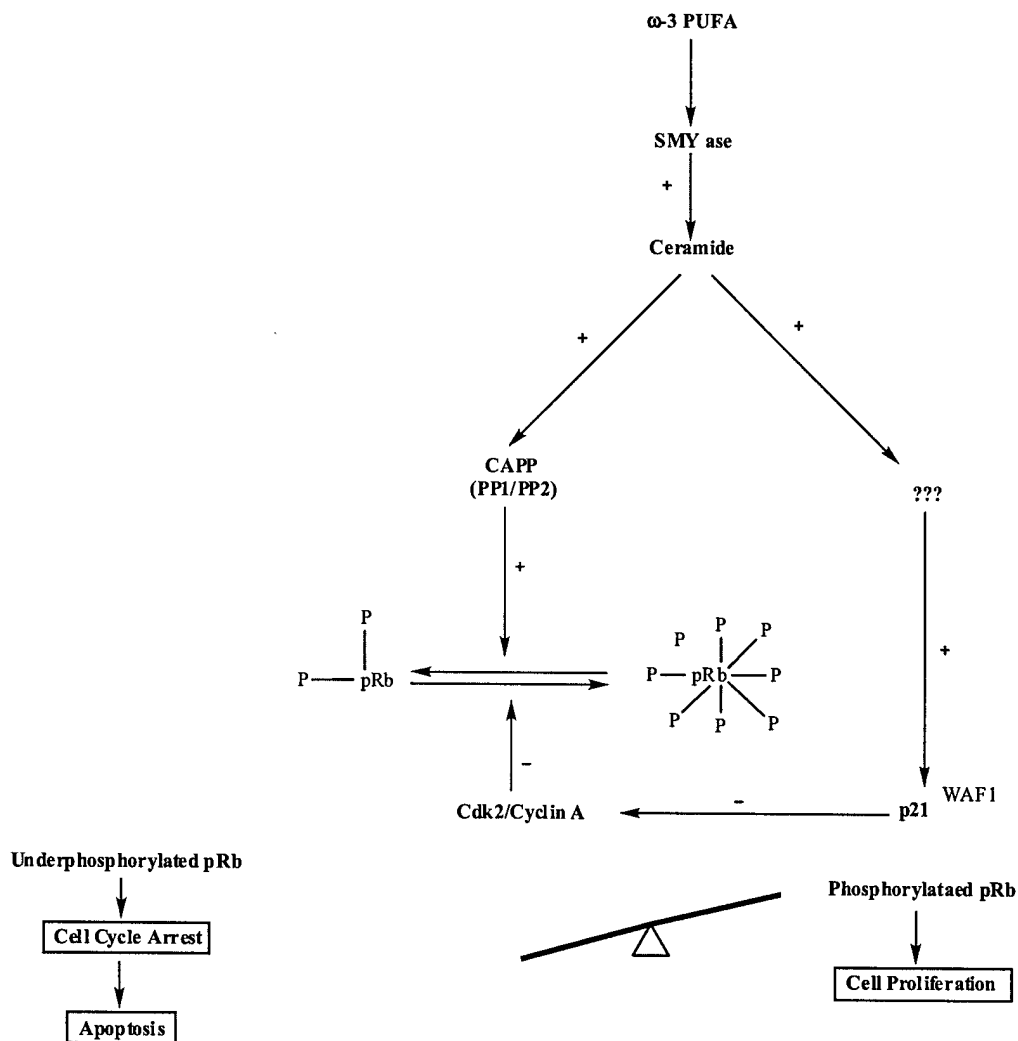
Fig. (4). Possible ω-3 PUFA-induced involvement of protein phosphatase in apoptosis. Activation of protein phosphatases by ω-3 PUFA-induced ceramide formation can affect cancer cell growth through multiple pathways. Via dephosphorylation of retinoblastoma protein (pRB) protein phosphatases cause cell cycle arrest, which then leads to the induction of apoptosis. Protein phosphatases can also mediate release of cytochrome c and activation of caspases via dephosphorylation of Bcl2/Bid proteins. However, it is also possible that protein phosphatases play a direct role in the activation of caspase 3. Activation of the executionary caspase 3 then leads to the induction of apoptosis.
