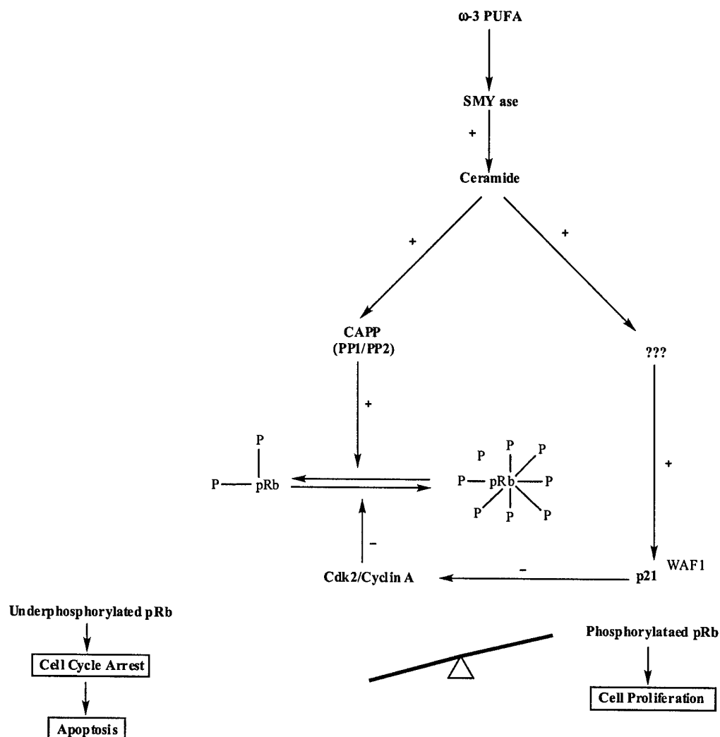
Fig. (3). Proposed action of \omega -3 PUFAs on cell cycle arrest in cancer cells
