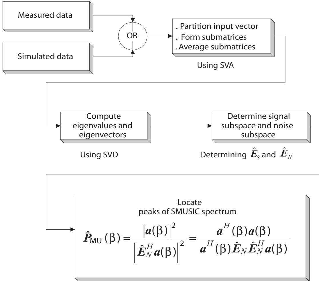
Figure 12: Ordinary SMUSIC process for experimental data and simulated data.
