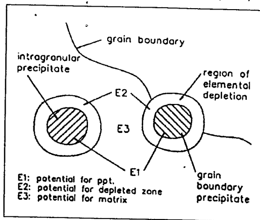
Figure 12: Depleted regions adjacent to precipitates. These regions cause an electrochemical potential difference that can promote localized corrosion at the microstructural level [1].
