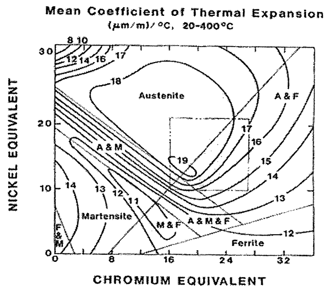
Figure 15: Mean coefficient thermal expansion ( \mu\text{m}/\text{m}/^\circ\text{C} , 20-400 ^\circ\text{C} ) plotted as isoexpansion contours on the Schaeffler constitution diagram [5].
