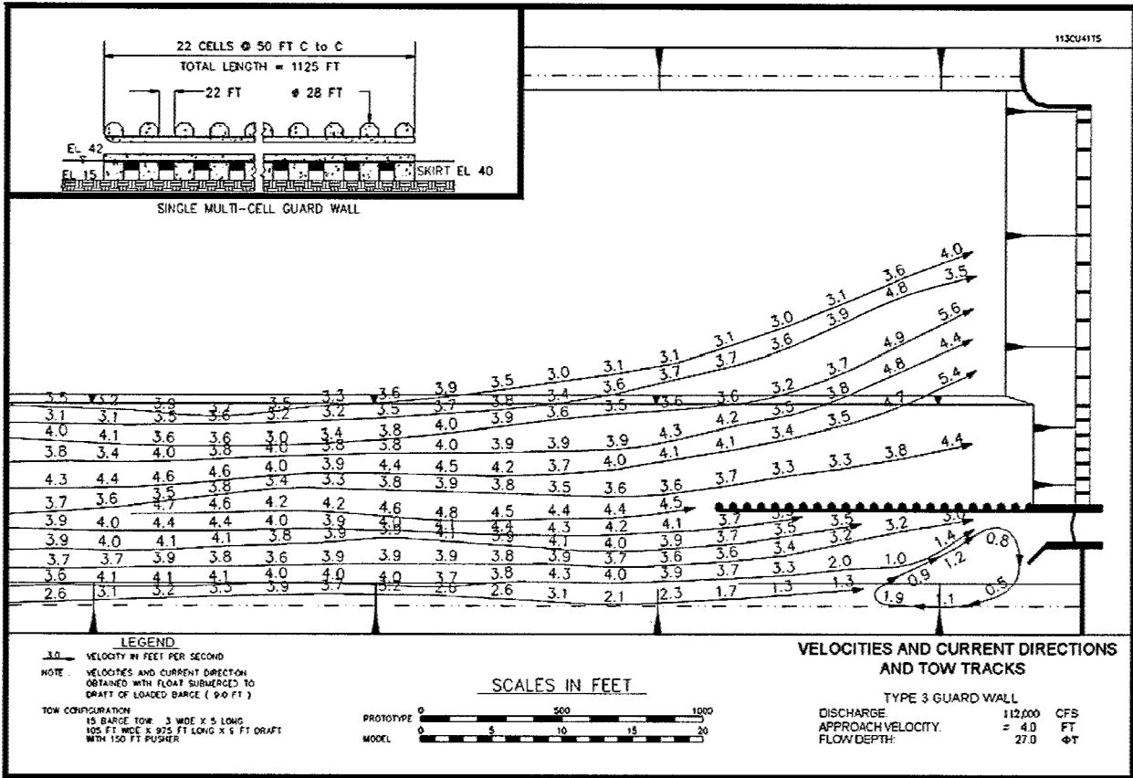
Figure 16. CDV and tow track data with type 3 guard wall
