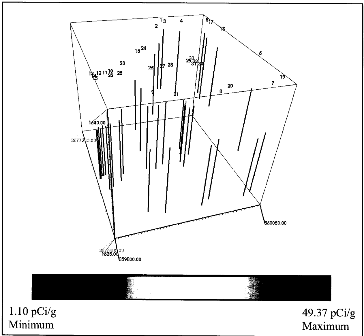
Figure 16. Thorium distribution in three dimensions. Elevated thorium activity levels were measured at only a few sampling sites near the helicopter at the center of the site
