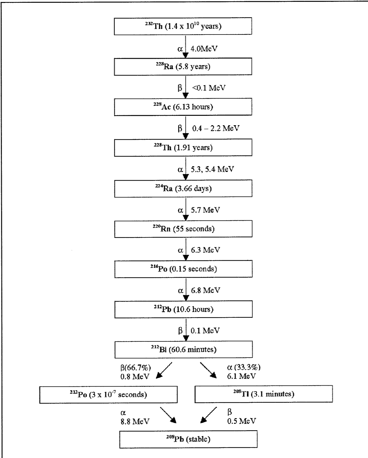
Figure 2. Thorium-232 decay series. Each elemental step is shown with the half-life following in parentheses. The type of decay (alpha ( \alpha ) or beta ( \beta )) is also shown along with the corresponding energy
