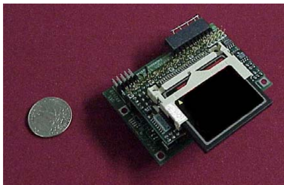
Figure 9 — Picture of the Persistor Inc. microprocessor board set with on board flash card.
