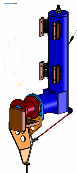
Figure 6 - Winch system with dynamic wire tensioning device and shock mounts.
