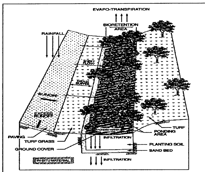
Figure 2: Bioretention Cell
