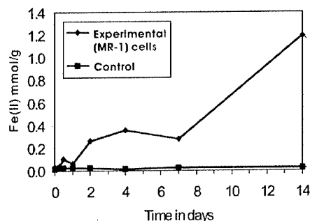
Fig. 1. Change of HCl-extractable Fe(II) with time in the Fe-rich smectite control and in the experimental (MR-1) tubes. The measured HCl-extractable Fe(II) concentration (mM) was normalized to milligrams of smectite in each tube and reported as mmol/g. The extent of reduction by the end of incubation reached 43%, based on measured Fe(III) concentration and the amount of smectite used in the tubes. The vertical errors are typically <10%.
