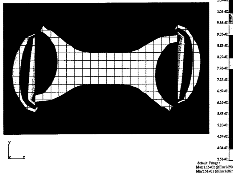
Figure 62 Von Mises stress for combined loading from (a) global model and (b) sub-model
