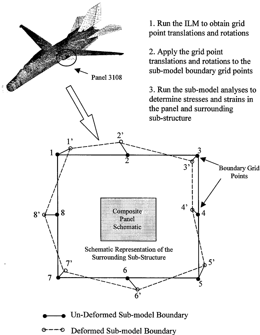
Figure 11 Sub-modelling methodology
