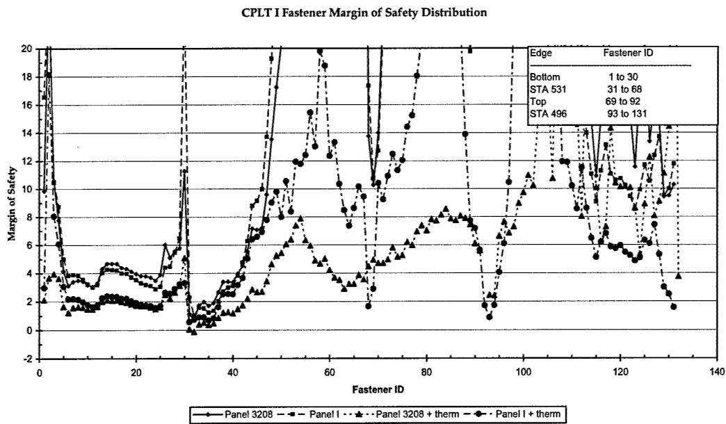
Figure 51 CPLT I fastener MOS distribution
