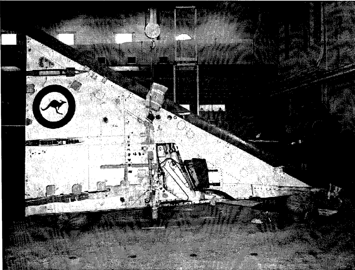
Figure 6: Lower Surface of Test Wing
