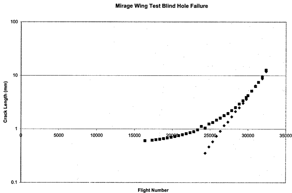
Figure 29: Fractographic Measurements versus Predicted Crack Growth (from Ref.37)
