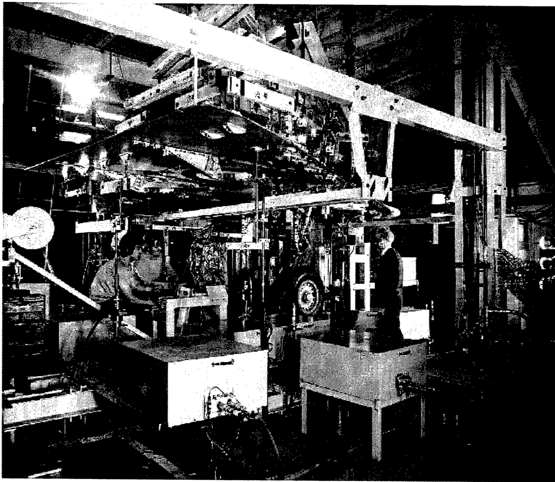
Figure 34: Wing Lower Surface showing Wing Removal Rails and Drag Load System
