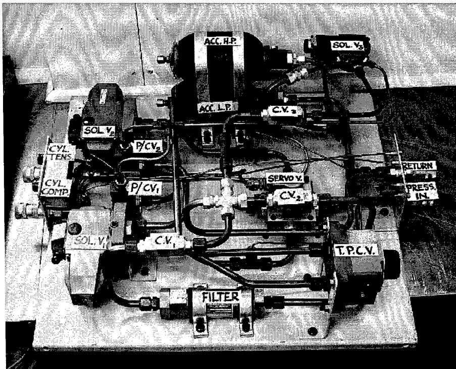
Figure 36: Actuator Control System (Valve Pack)
