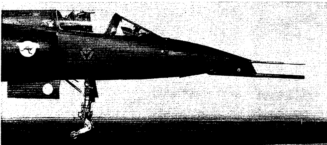
Figure 3: Gust Probe Mounted to Flight Trials Aircraft
