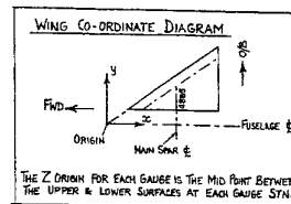
Figure 8: Mirage Wing Instrumentation (See Appendix A for gauge descriptions)
