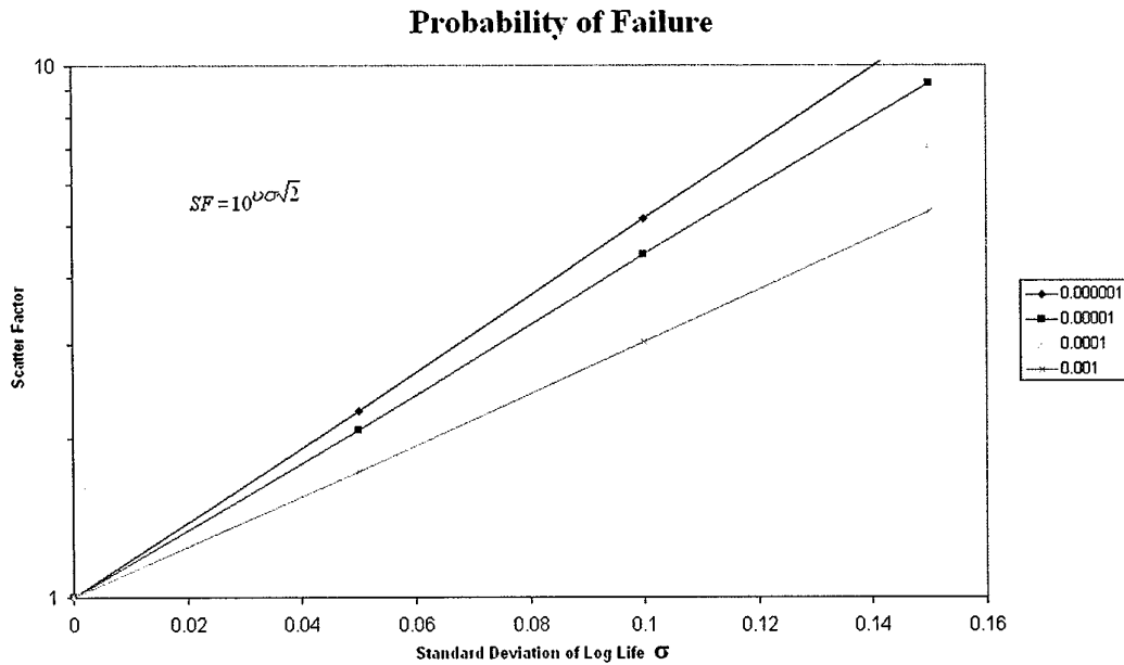
Figure 37: Scatter Factors versus Probability of Failure
