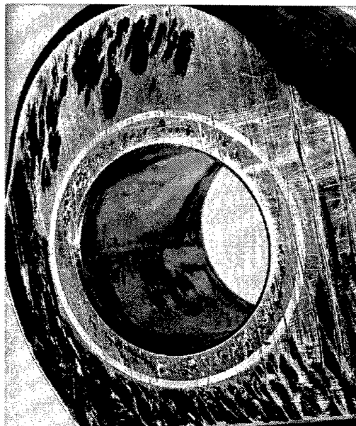
Figure 35: Lower Hole, Forward Face after Completion of Test
