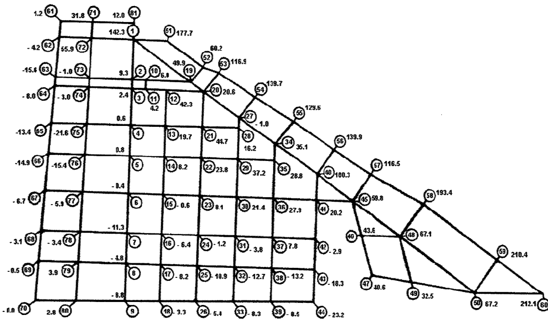
Figure 18: Level Flight Load Distribution (1g) Used as a base for Gust Loads (kg)
