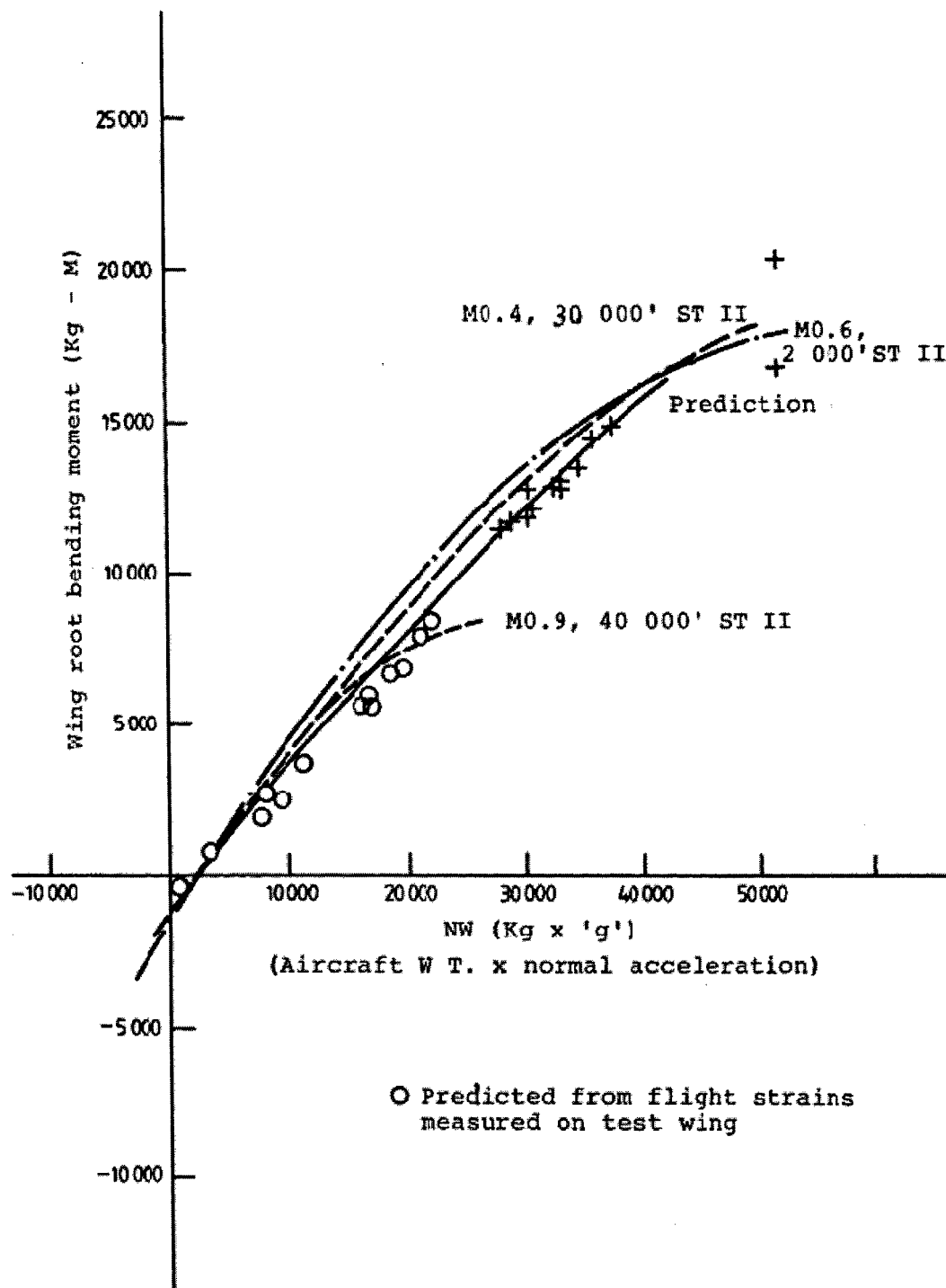
Figure 15: Wing Root Bending Moment Predictions
