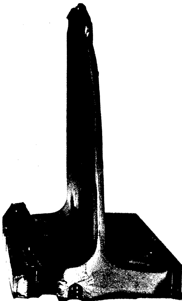
Figure 27: General View of the Final Failure in the Main Spar Lower Flange
