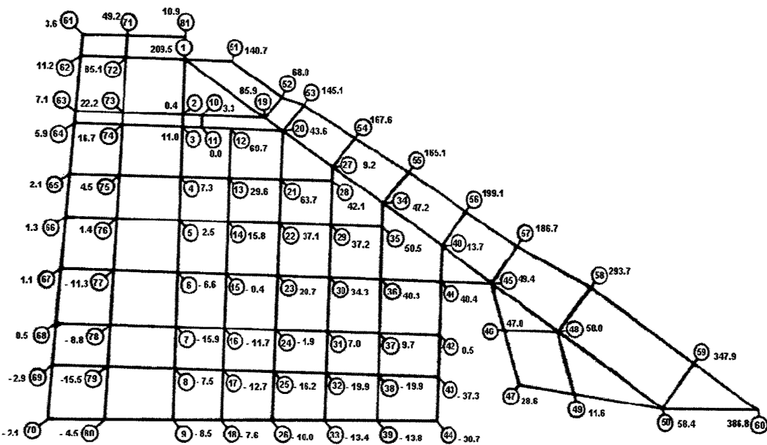
Figure 19: Estimated Distribution of Load per g due to Gusts (kg)
