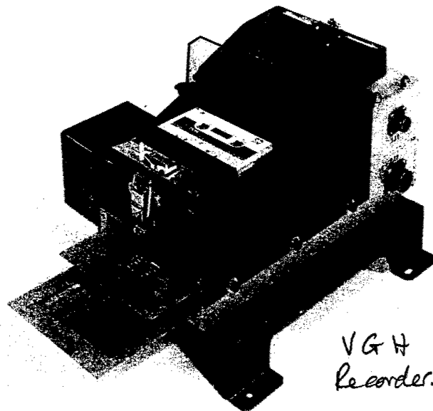
Figure 2: ARL Designed V-g-H Cassette Tape Recorder for Mirage Gust Load Studies
