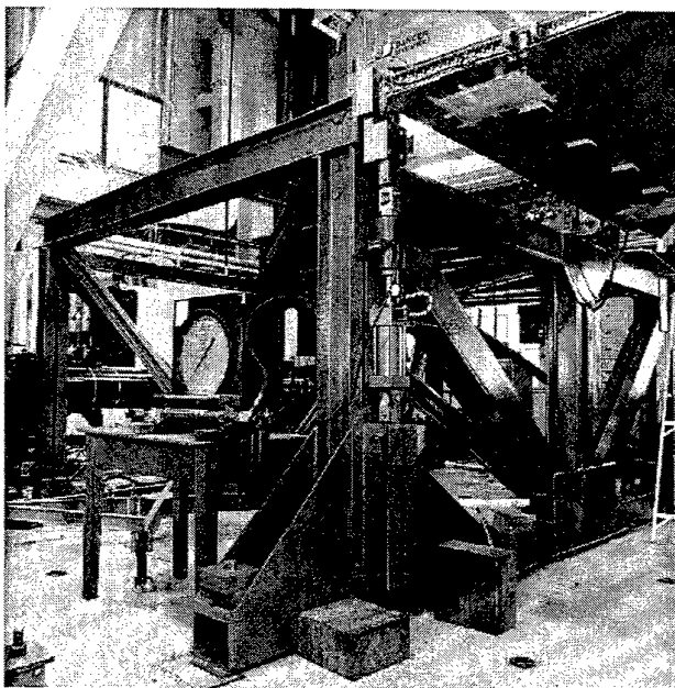
Figure 30: Wing Test Rig Dummy Fuselage Showing Two of Four Attachment Locations
