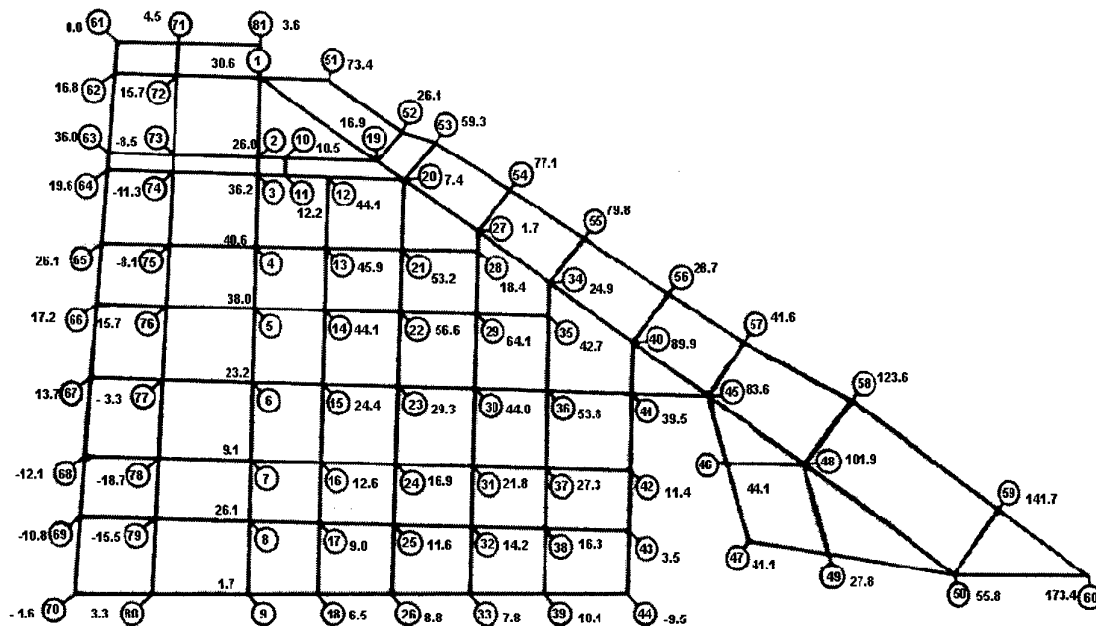
Figure 20: Load Distribution to Represent Wing Loads during Loading
