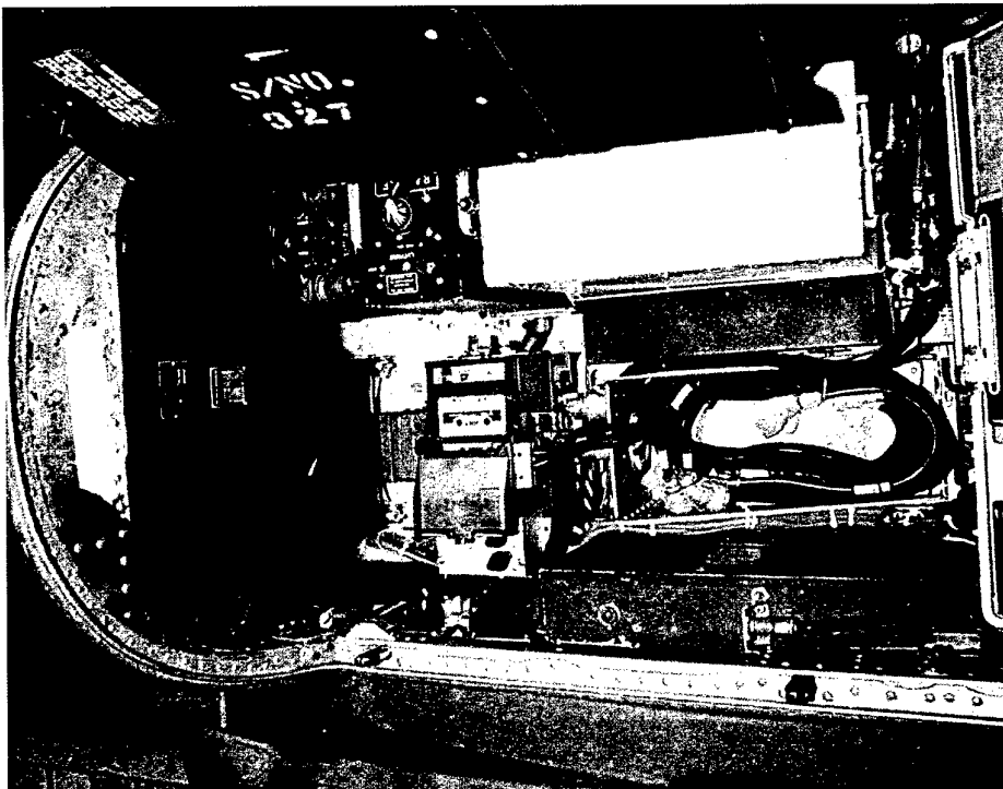
Figure 13: AFDRAS Recorder in Rear Bay of Mirage
