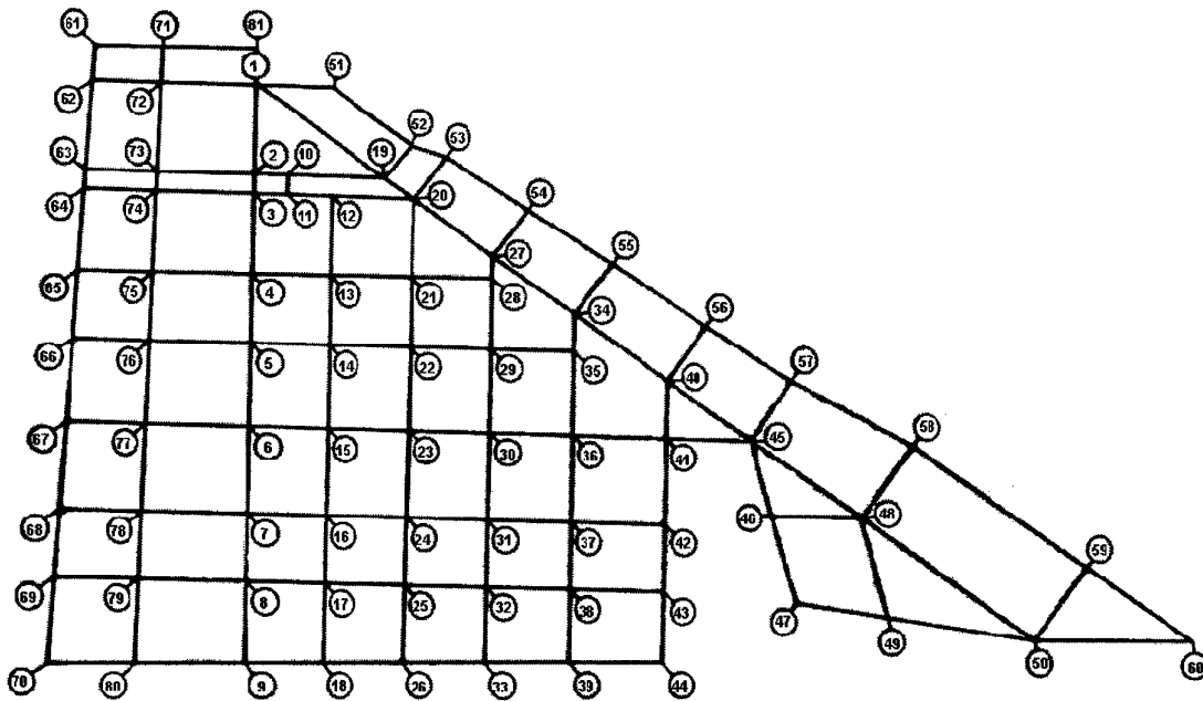
Figure 16: Nodal Point Representation of Wing and Elevon
