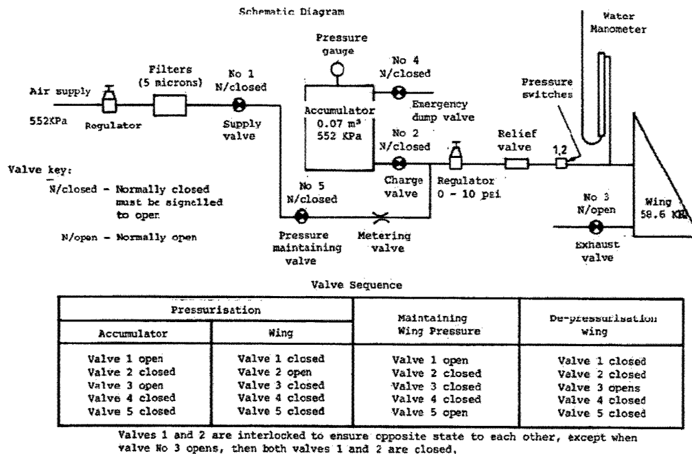
Figure 23: Pressurisation Schematic of Wing Fuel Tank
