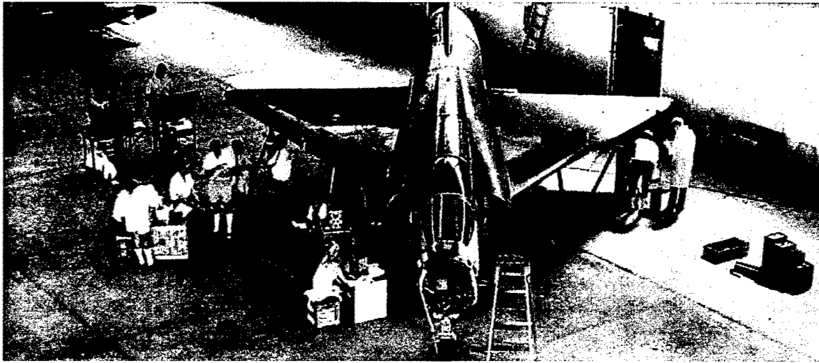
Figure 11: Test Aircraft Ground Calibration
