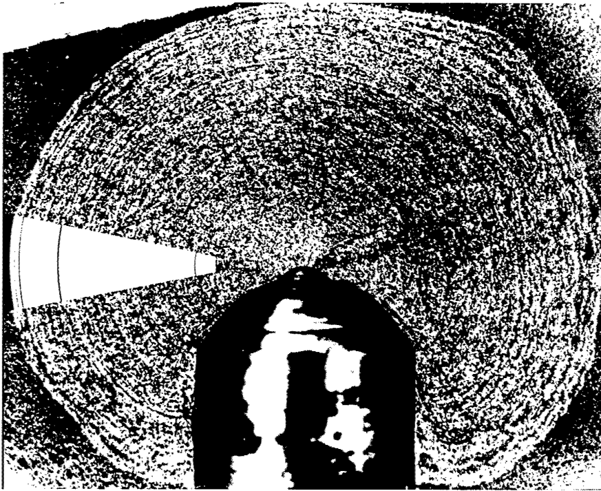
Figure 28: Close-up View of Failure Location showing Fatigue Crack Progression Markings and those Predicted by Quantitative Fractography
