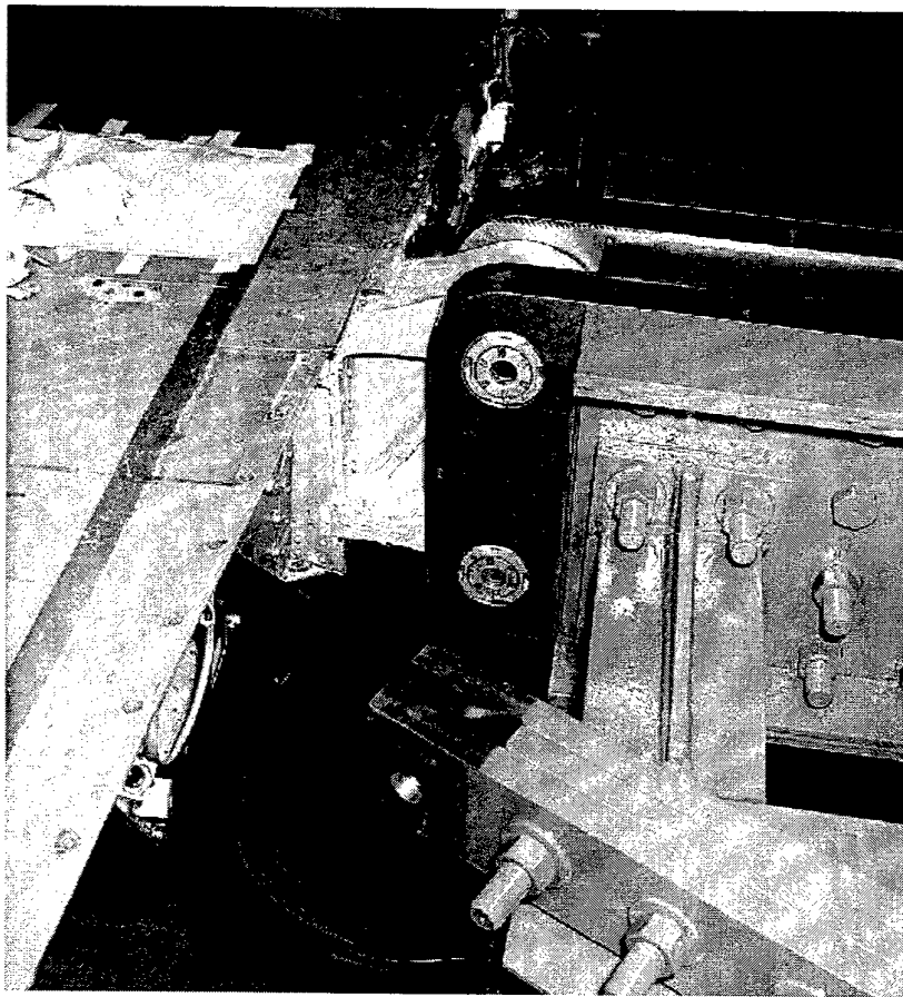
Figure 32: Main Spar and Undercarriage Side Link Attachment Points on Dummy Fuselage
