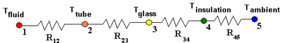
Figure 11, Resistance Model
