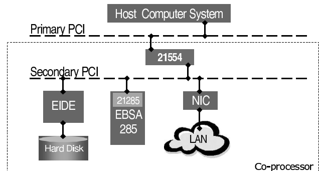
Figure 2. Detailed Diagram of CiNIC Architecture
