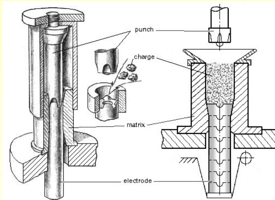
Scheme of electrode pressing
