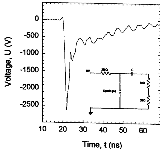
Fig. 7a. Pulse obtained without diode
