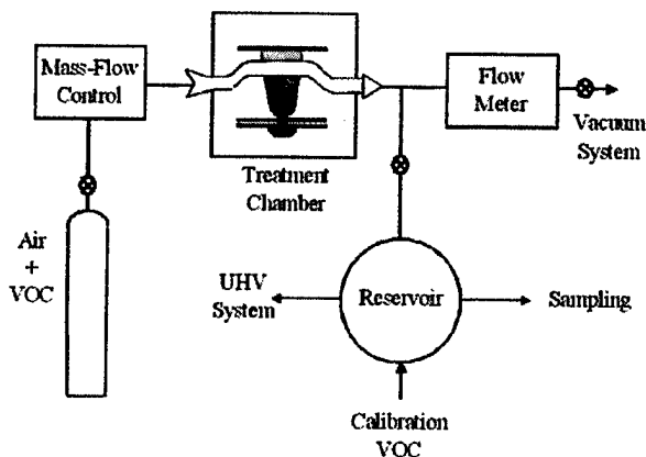
Fig 3(b) schematic diagram of the experimental setup
