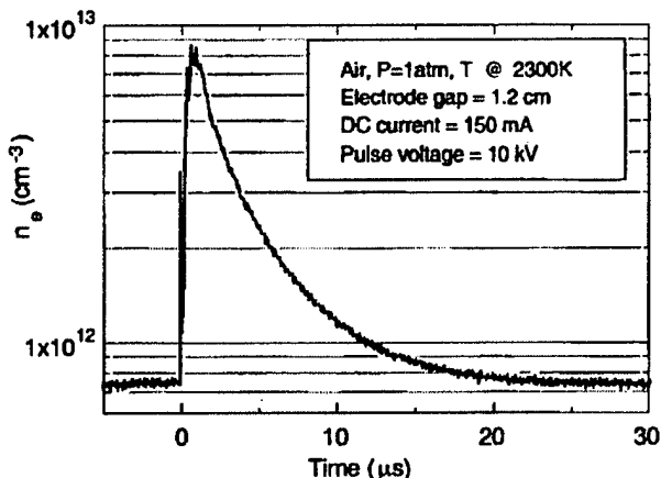
FIGURE 6. Electron number density as a function of time for the pulsed discharge experiment.
