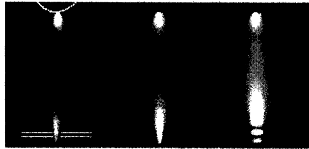
Fig. 1. Photographs of atmospheric pressure air glow discharges at currents of 5.3, 11.1, and 22 mA (from left to right). The electrodes are shown schematically in the photograph on the left.
