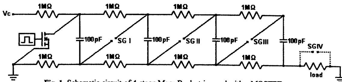
Fig. 1. Schematic circuit of 4-stage Marx Bank, triggered with a MOSFET
