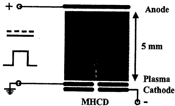
Fig. 1 Photograph of a microhollow cathode discharge sustained in xenon at 100 torr and a 2 mA discharge current. In order to study the electron heating effect, a 10 ns high voltage pulse was superimposed to the dc plasma.
