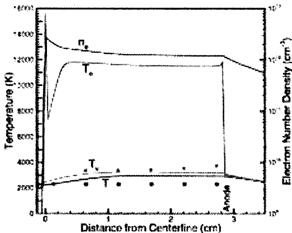
FIGURE 9. Computed electron number density and temperatures along the DC discharge centerline. Symbols denote experimentally measured values.
