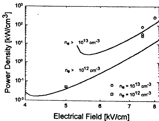
Figure 9. Power density versus the applied electrical field for different electron densities. The solid lines represent the modeling results, circles and squares represent measured values.
