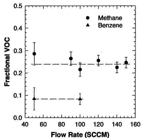
Figure 8 Methane and benzene dynamics: (a) fractional VOC versus flow rate, and (b) fractional VOC versus residence time at a discharge voltage of 470 V. The discharge current was 17 mA for methane/dry air, and 14 mA for benzene/dry air.
