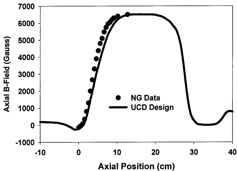
Fig. 4.1.13 Design axial magnetic field profile compared to the Northrop Grumman recommended field.
