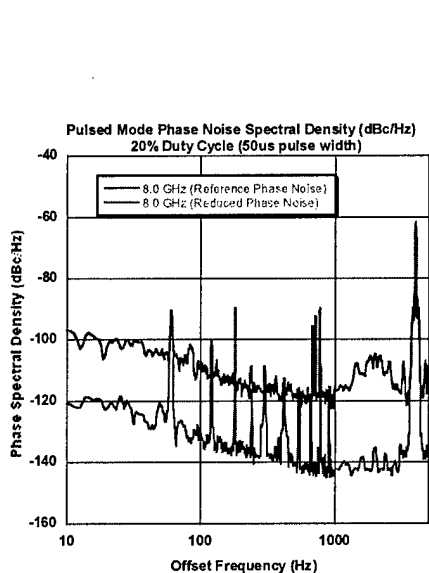
Fig. 4.1.36 Phase noise measured for pulsed mode operation with 20% duty cycle (50 \mu s pulse), carrier frequency is 8GHz
