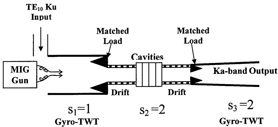
Fig. 4.5.10 Schematic of Frequency Doubling Gyro-TWT
