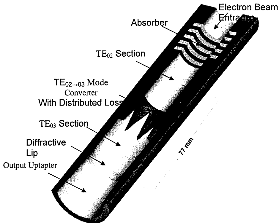
Fig. 4.5.3 35 GHz Multi-Mode Resonant Cavity
