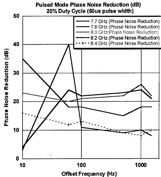
Fig. 4.1.37 Phase noise reduction for pulsed mode with 20% duty cycle (50 \mu s pulse) carrier frequency from 7.7~8.4 GHz
