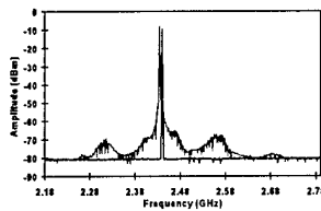
UM-Demonstrated Noise Suppression in a magnetron
