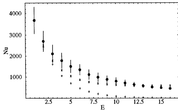
Fig. 1. The number of unchanged genes as a function of the number of samples for the Perou et al. (1999) data set. The curves show the the expected number of unchanged genes based on (8), assuming that all genes can be changed (lower curve, + symbols) or that only 5100 genes are changeable (X symbols). The dots with error bars show the results from the experimental data. The error bars stem from the fact that, for the data point corresponding to e samples, there are \binom{E}{e} ways of selecting the samples.
