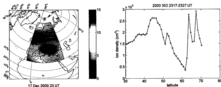
Figure 3.8a. MIDAS image of the vertical TEC across the ionosphere over Europe and b. ion density from the (northward) CHAMP satellite orbiting between 17° and 20° longitude.
