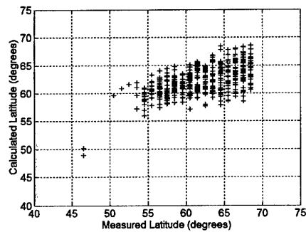
Figure 5.3. Measured and calculated trough position for Model C of Table 5.1.
