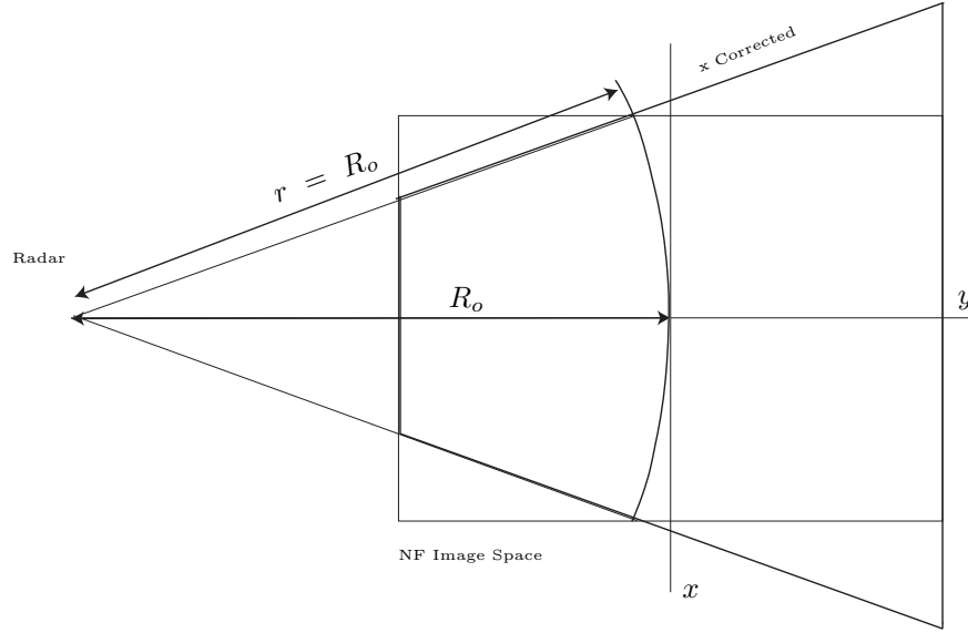
Figure 5.10: The original cross-range and downrange extents are defined by the rectangular boundary. Cross-range extent correction redefines a trapezoidal boundary. This compression and expansion in the boundary results from shorter and longer, respectively, propagation distances, r , with respect to, R_o . The curved contour is points where r = R_o . At these points the original cross-range extent is equal to the new cross-range extent.
