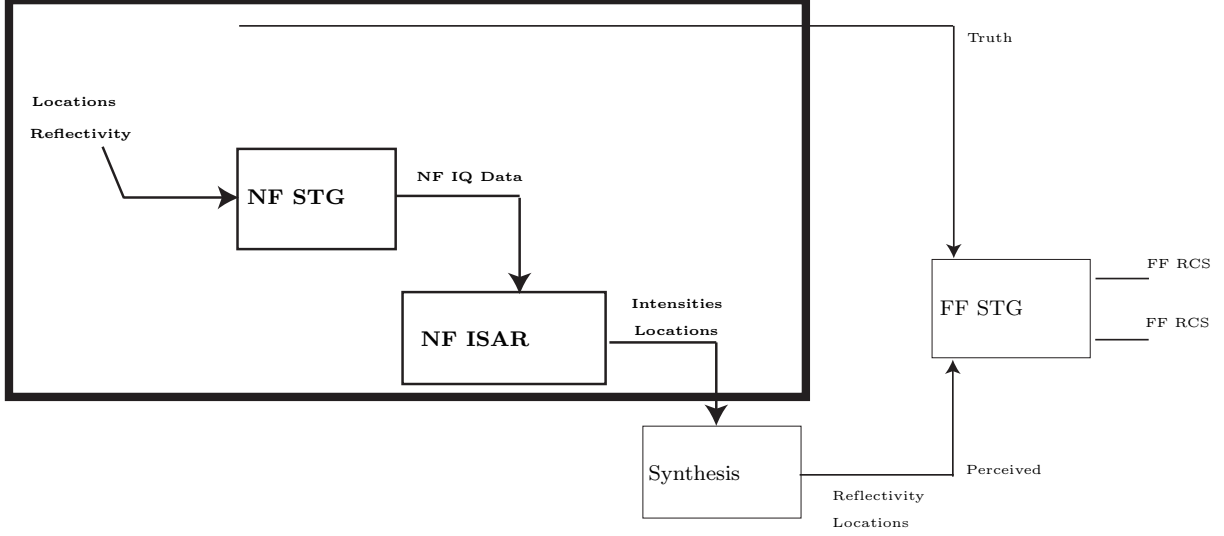
Figure 4.2: The primary focus in this Near-Field to Far-Field Transformation is on developing a spatially accurate NF ISAR image. This focuses on the NF STG and ISAR process. The entire process is describe by starting with the two ISAR Synthetic Target Generators (STGs) that take real scattering center locations and reflectivities and create FF and NF IQ Data. The FF IQ data is considered truth data. The NF IQ Data is imaged by an ISAR code, mapping maximum intensity spatial locations. These complex intensities extracted by scattering center synthesis provide spatial locations and relative phases. These locations and complex amplitudes are passed through a FF STG producing a FF RCS. This FF RCS is compared to the true FF RCS generated from the real locations.
