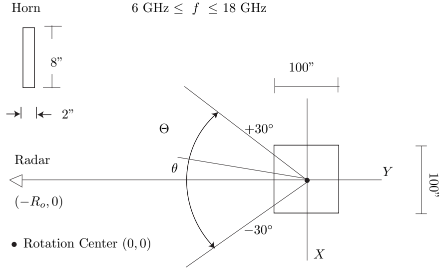
Figure 4.1: A 100" \times 100" extent measured at a radar to target rotation center distance R_o = 155' . The target is rotated through a 60° azimuth in 0.06° increments and scattering centers are illuminated synthetically by the specified bandwidth within this area.
