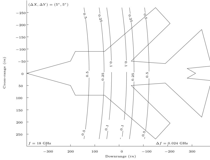
Figure G.2: Nyquist sampling determines the downrange imageable extent without aliasing. Therefore, the number of cycles per frequency sample can not exceed 0.5. The contours represent cycles per 0.024 GHz frequency increment at a max frequency, f = 18 GHz. Since, the 0.5 contours do not circumscribe the entire target, this example is not sampled finely enough to satisfy the Nyquist criteria over the full aircraft extent.
