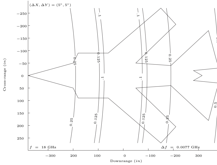
Figure G.3: Nyquist sampling determines the downrange imageable extent without aliasing. Therefore, the number of cycles per frequency sample can not exceed 0.5. The contours represent cycles per 0.0077 GHz frequency increment at a max frequency, f = 18 GHz. Since the contours fully circumscribe the target this example is sampled finely enough to satisfy the Nyquist criteria over the full aircraft extent.
