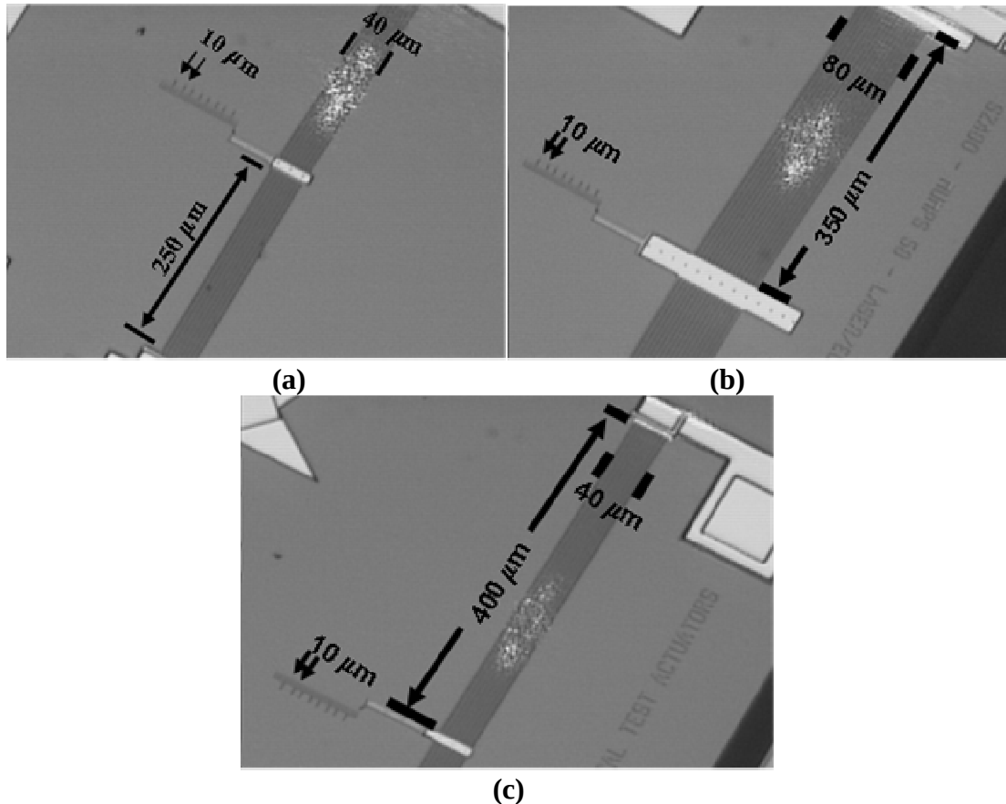
Figure 4.9: Digital photographs, showing PolyMUMPs 58 test actuators under laser testing, with (a) 250 \mu\text{m} by 8-beam chevron, (b) showing a 350 \mu\text{m} by 16-beam chevron and (c) showing a 400 \mu\text{m} by 8-beam chevron.
