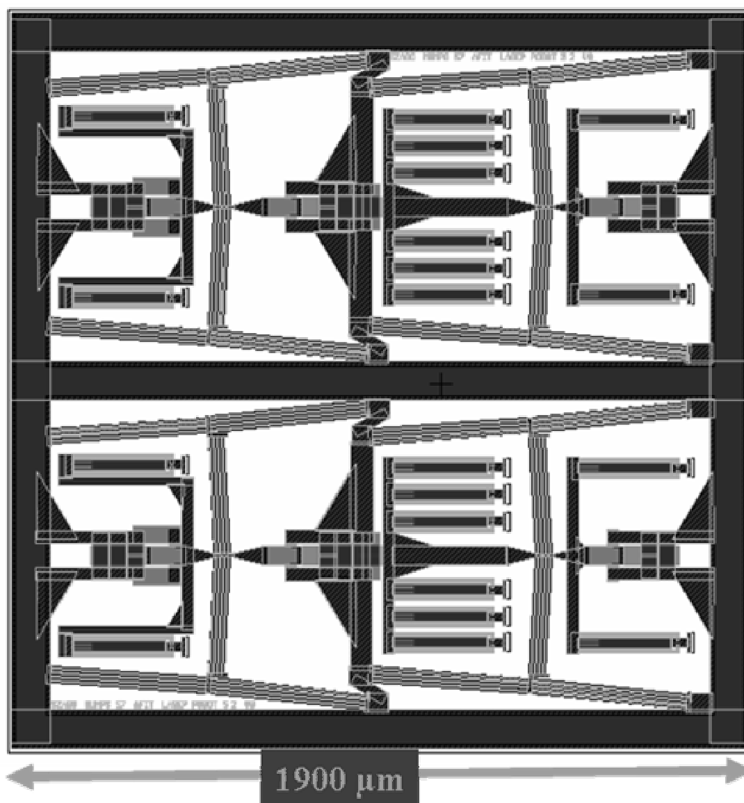
Figure A1.6: L-Edit layout showing the PolyMUMPs 57 microrobot design; a cascade-microrobot design with a 1900 by 1900 \mu\text{m} size, 400 and 300 \mu\text{m} long chevron actuators with 4 chevron beams, and with twenty, 250 \mu\text{m} long down thermal actuators.
