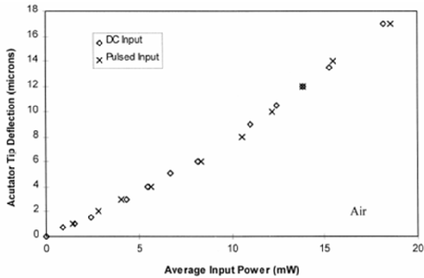
Figure 5.2: Plot of experimental data of electrical power versus deflection for single asymmetrical hot arm electrothermal actuators obtained by Cowan, et al. [2].
