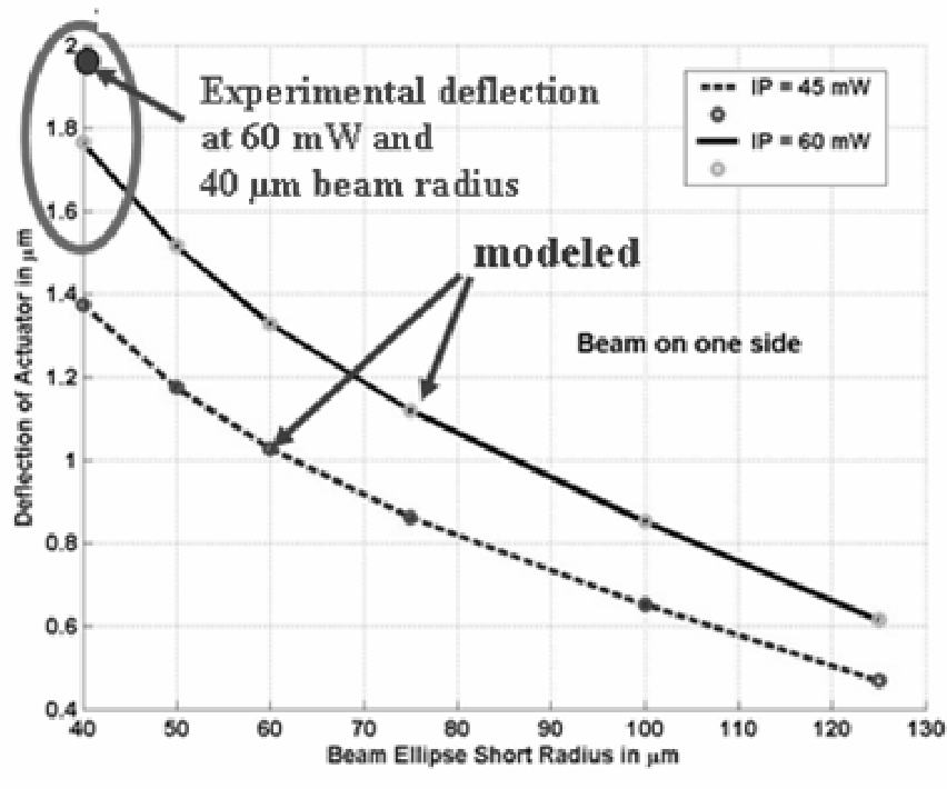
Figure 7.20: Plot showing the model predicted deflection versus laser beam dot size with the beam asymmetrical heating one side of actuator and giving almost 2 \mu\text{m} of deflection at 60 mW of incident power and a 40 \mu\text{m} beam dot radius.
