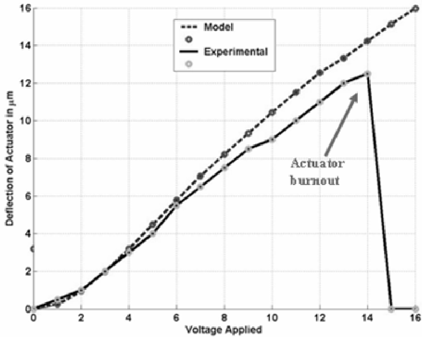
Figure 5.8: Example plot of deflection obtained from the model as compared to experimental deflection of an electrically powered 250 \mu\text{m} by 8-beam chevron actuator designed for the PolyMUMPs 58 fabrication run.
