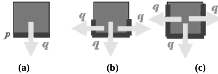
Figure 5.6: Illustration of the three cases of calculating perimeter, P , for the convective heat loss, q , with (a) having P = length of the bottom, and (b) having P = length of the bottom plus half the sides, and (c) having P = length of the bottom plus the length of both sides.
