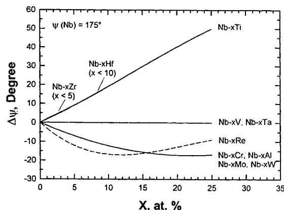
Figure 6. Change of the lattice phase angle \Delta\psi = \psi(\text{Nb-X}) - \psi(\text{Nb}) , as a function of alloying addition for various Nb-X binary alloys. Ductilizing elements (Ti, Hf, and Zr) increases the lattice phase angle ( \Delta\psi > 0 ), while embrittling elements (Cr, Al, Mo, W, and Re) decreases the lattice phase angle ( \Delta\psi < 0 ).
