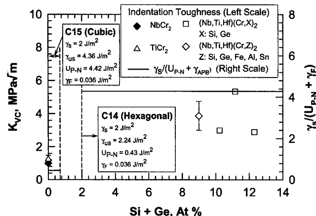
Fig. 16—Fracture toughness, unstable stacking energy ( \gamma_{us} ), P-N barrier energy ( U_{P-N} ), and crystal structure of Laves phase as a function of Si and Ge addition.
