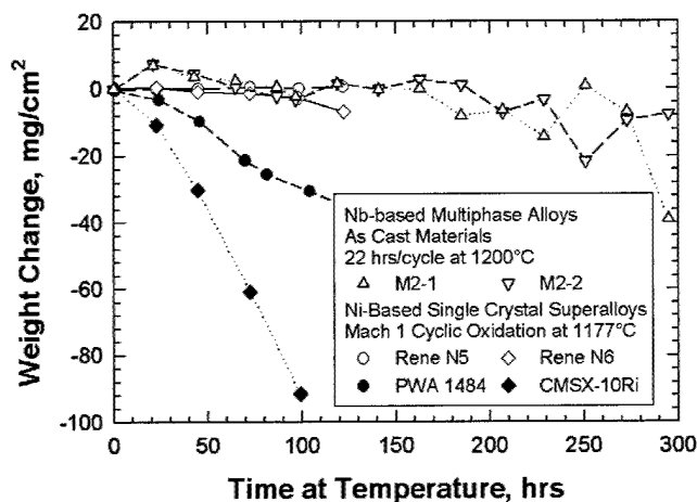
Fig. 10—A comparison of the weight change curves of the Nb-based multiphase alloy M2 (M2-1 and M2-2 are duplicate specimens) from this study against those of four Ni-based single-crystal superalloys, which are RENE N5, RENE N6, PWA 1484, and CMSX-10Ri, from Walston et al. [47]
