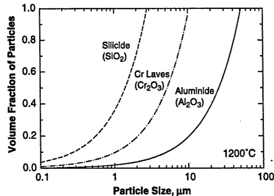
Fig. 5. Model calculations of the critical volume fraction of particles as a function of particle size (diameter) for forming a protective-oxide layer of \text{SiO}_2 , \text{Cr}_2\text{O}_3 , and \text{Al}_2\text{O}_3 for silicide, Cr Laves phase, and aluminide particles, respectively, after 2 hr exposure at 1200^\circ\text{C} .
