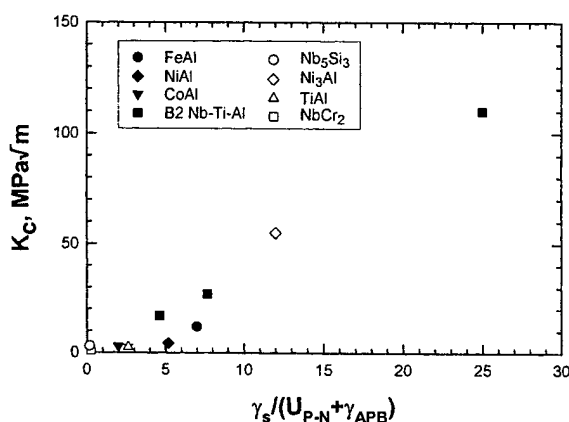
Figure 5. Increasing fracture toughness ( K_C ) with increasing values of the ductility index defined in terms of the \gamma_S/(U_{P-N}+\gamma_{APB}) ratio for various intermetallics.
