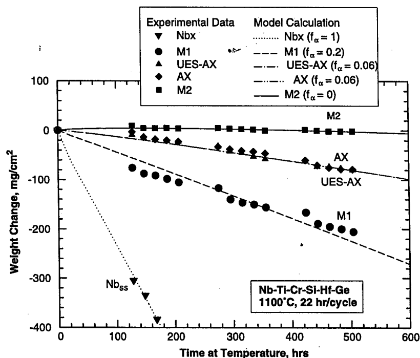
Fig. 10. Comparison of measured and computed weight-change curves for Nb-base in situ composites. The model was fitted to the experimental weight change data to deduce the area fractions ( f_\alpha ) of Nb solid-solution phases covered by \text{Nb}_2\text{O}_5 \cdot \text{TiO}_2 for M1, UES-AX and AX. The deduced values f_\alpha for these alloys are significantly lower than the volume fraction of the Nb solid-solution phase, which suggests that there is a tendency to form \text{CrNbO}_4 at the expense of \text{Nb}_2\text{O}_5 \cdot \text{TiO}_2 .
