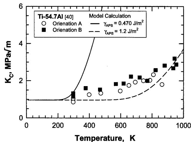
Fig. 6—Computed K_{IC} compared against experimental data of binary TiAl (Ti-54.7Al) [40] as a function of temperature. The fracture model overpredicted the fracture toughness when the experimental \gamma_{APB} value ( 0.47 \text{ J/m}^2 ) [46] was used. The \gamma_{APB} required to fit the model to the data was 1.2 \text{ J/m}^2 . The high apparent \gamma_{APB} value suggests that dislocation nucleation at the crack tip might be the controlling slip mechanism.
