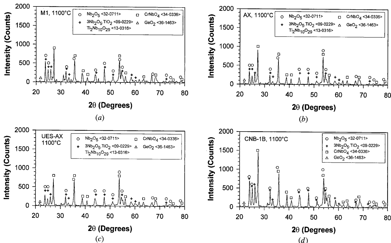
Fig. 7—Characteristic XRD peaks of oxide spalls of four Nb-based multiphase alloys ((a) M1, (b) AX, (c) UES-AX, and (d) CNB-1B) tested at a peak oxidation temperature of 1100 °C.
