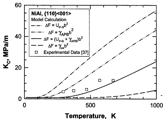
Fig. 5—Dependence of computed K_{IC} on individual dislocation barriers for \{110\}\langle 001 \rangle slip in NiAl. The K_{IC} increases with decreasing barrier energy since U_{P-N} < \gamma_{APB} < \gamma_{us} .
