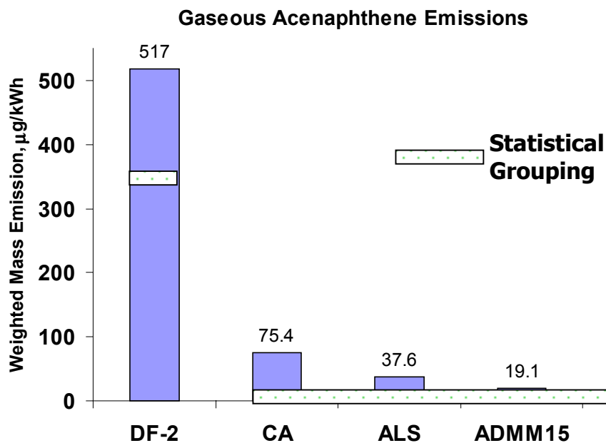
Figure 38. Test Fuel Weighted Average Gaseous Phase Acenaphthene Mass Emissions ( \mu\text{g/kWh} )
