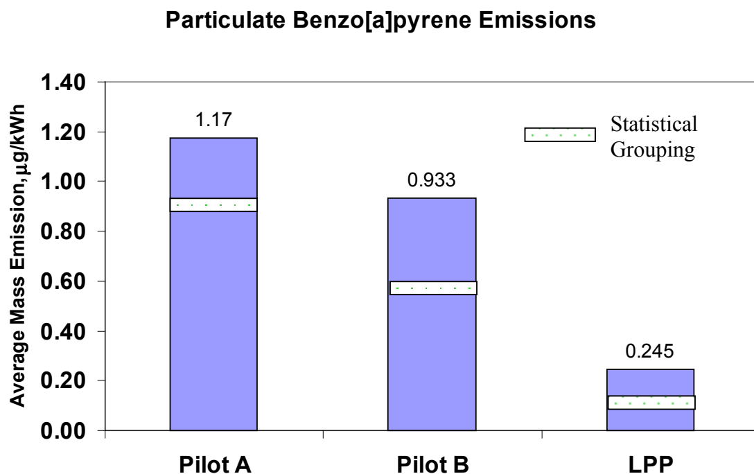
Figure 94. Pilot Condition Average Particulate Phase Benzo[a]pyrene Mass Emissions for Test Fuels and Modes (µg/kWh)
