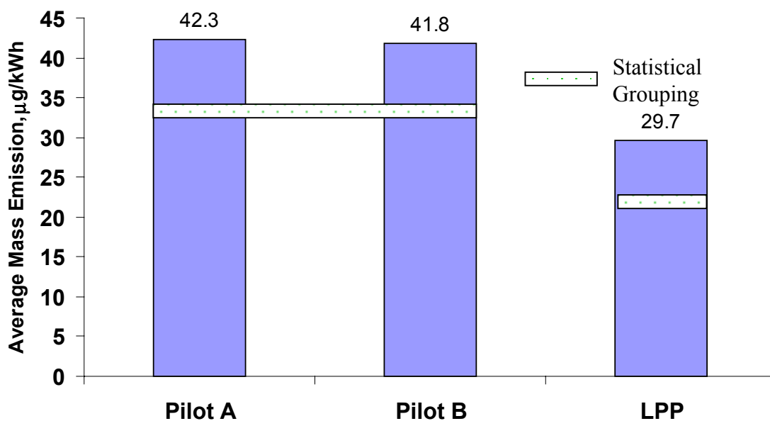
Figure 82. Pilot Condition Average Particulate Phase Pyrene Mass Emissions for Test Fuels and Modes (µg/kWh)
