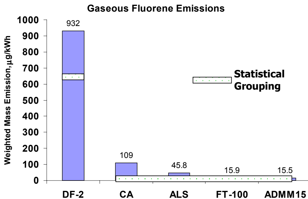
Figure 39. Test Fuel Weighted Average Gaseous Phase Fluorene Mass Emissions ( \mu\text{g/kWh} )
