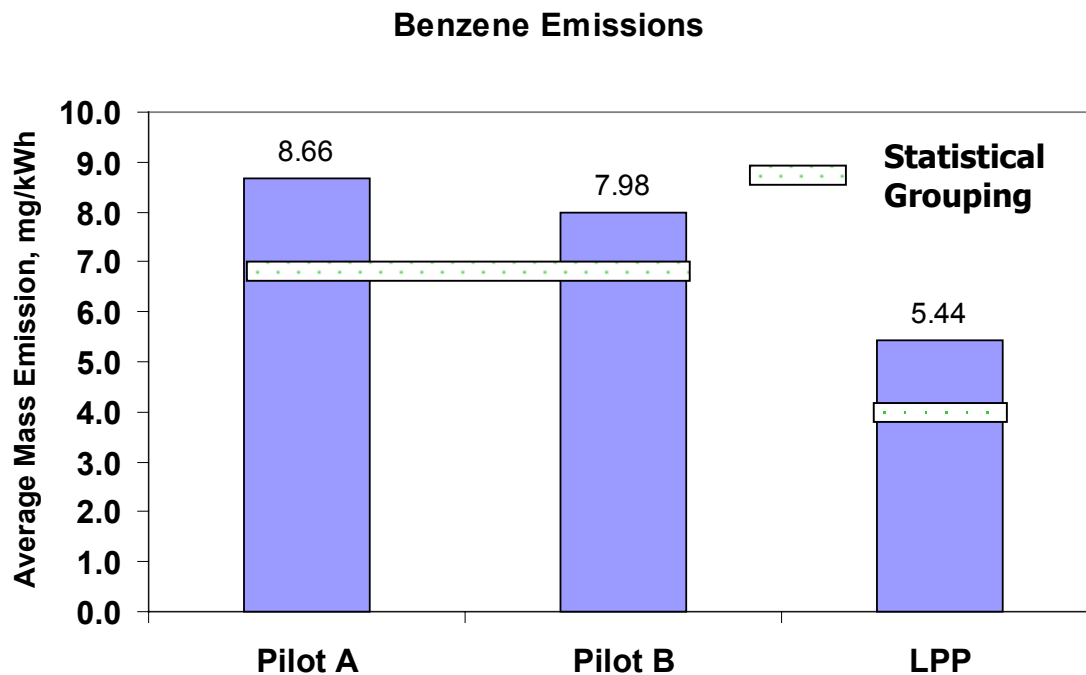
Figure 60. Pilot Condition Average Benzene Mass Emissions for Test Fuels and Modes (mg/kWh)
