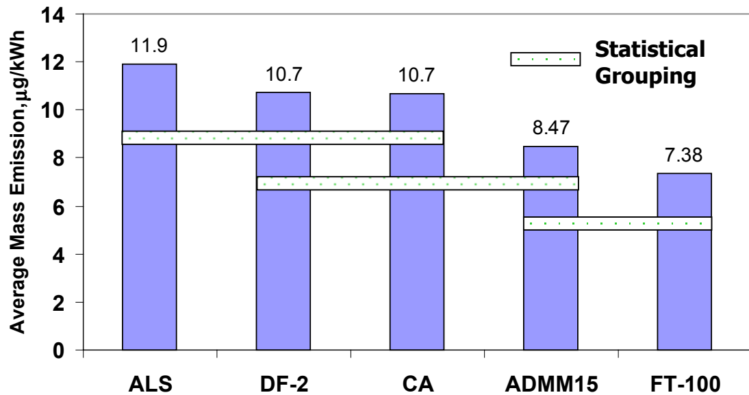
Figure 73. Test Fuel Average Particulate Phase Fluorene Mass Emissions for Pilot Conditions and Modes (µg/kWh)
