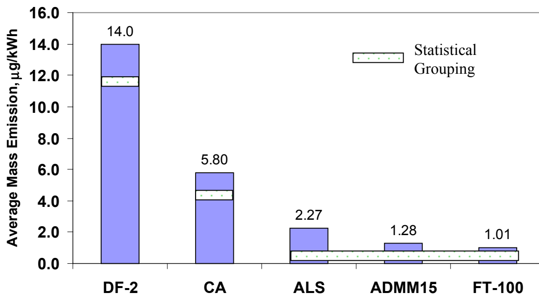
Figure 85. Test Fuel Average Particulate Phase Chrysene Mass Emissions for Pilot Conditions and Modes ( \mu\text{g/kWh} )
