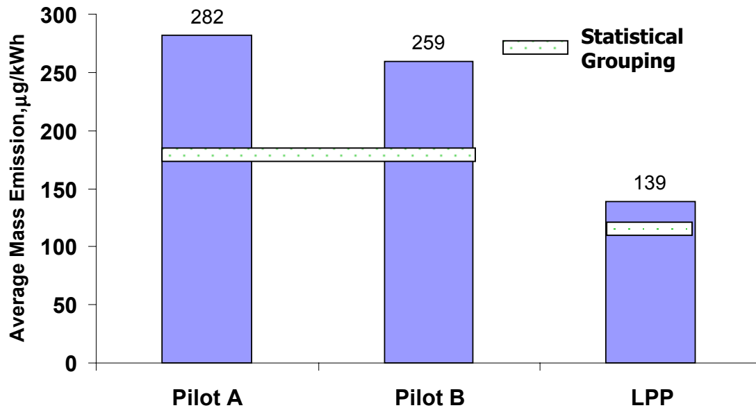
Figure 108. Pilot Condition Average Gaseous Phase Acenaphthylene Mass Emissions for Test Fuels and Modes (µg/kWh)
