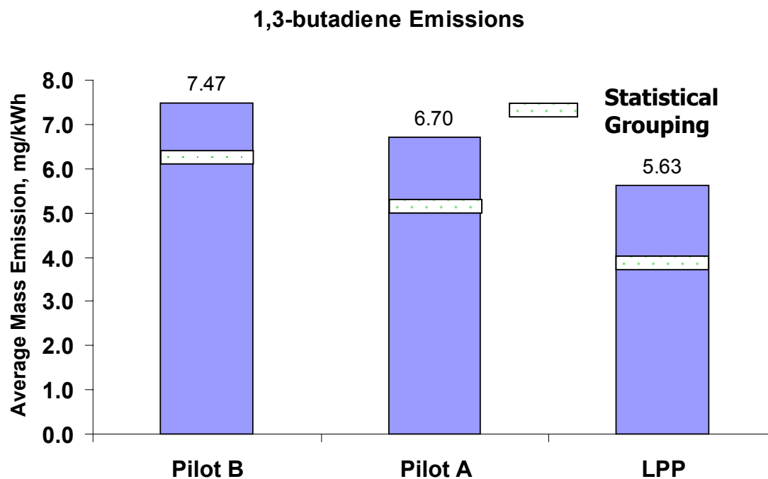
Figure 62. Pilot Condition Average 1,3-butadiene Mass Emissions for Test Fuels and Modes (mg/kWh)
