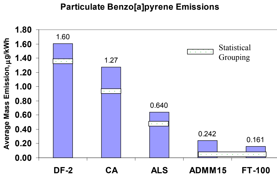
Figure 93. Test Fuel Average Particulate Phase Benzo[a]pyrene Mass Emissions for Pilot Conditions and Modes (µg/kWh)
