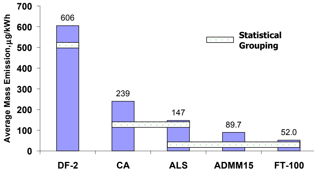
Figure 107. Test Fuel Average Gaseous Phase Acenaphthylene Mass Emissions for Pilot Conditions and Modes (µg/kWh)
