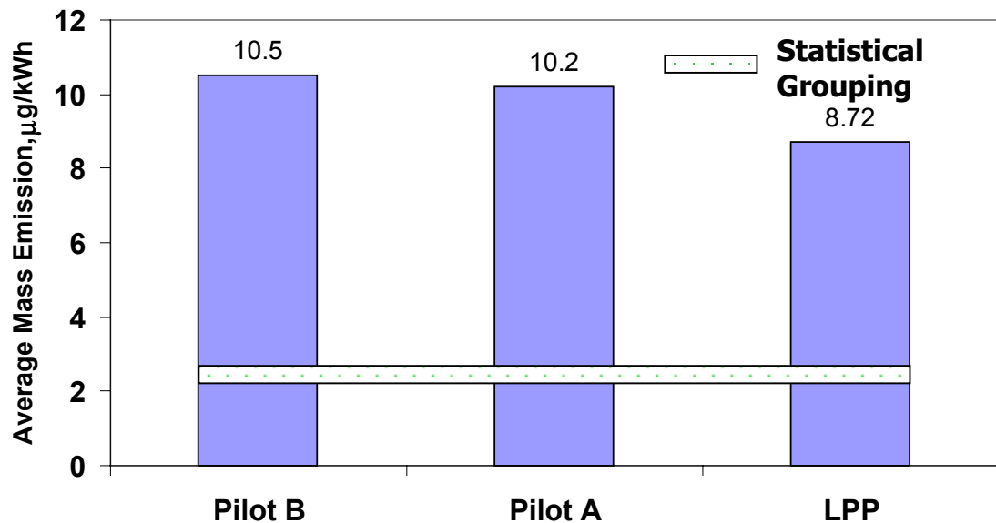
Figure 74. Pilot Condition Average Particulate Phase Fluorene Mass Emissions for Test Fuels and Modes (µg/kWh)
