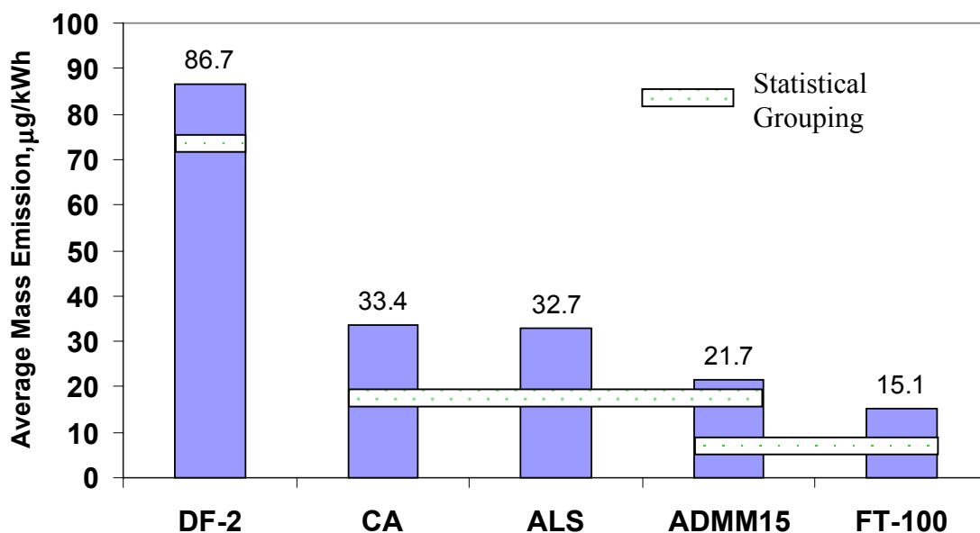
Figure 81. Test Fuel Average Particulate Phase Pyrene Mass Emissions for Pilot Conditions and Modes (µg/kWh)
