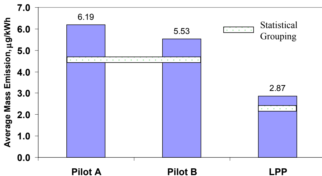
Figure 86. Pilot Condition Average Particulate Phase Chrysene Mass Emissions for Test Fuels and Modes ( \mu\text{g/kWh} )
