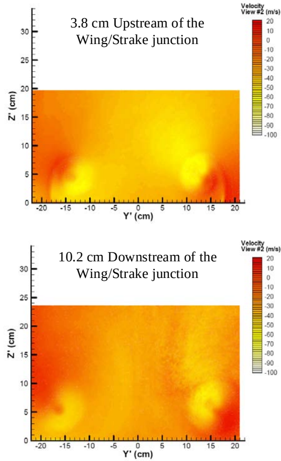
Figure 5.39 PDV measurement of Boeing interference model at an angle of attack of 20 degrees measured 3.8 cm and 10.2 cm upstream and downstream of wing strike junction. The system sensitivity unit vector for this side view is (-0.304i, 0.406j, 0.848k) .
