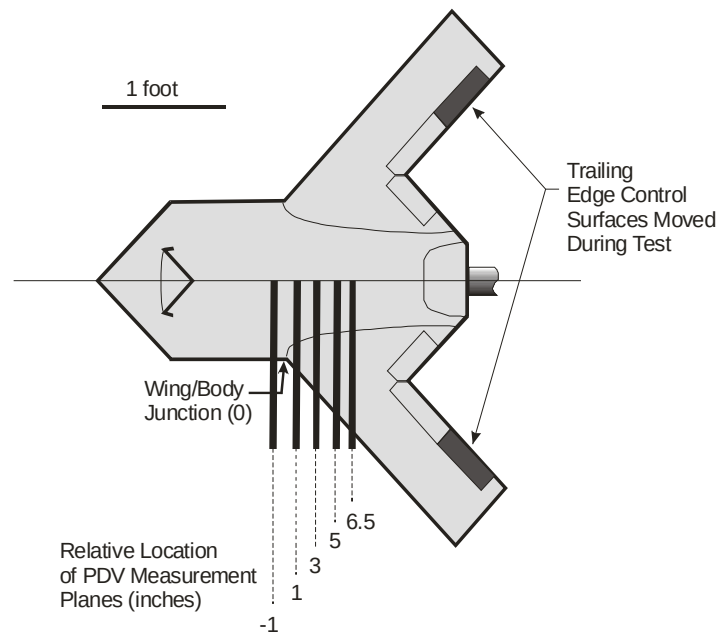
Figure 5.43 Schematic of Boeing UCAV model used in 3-D PDV tests.
