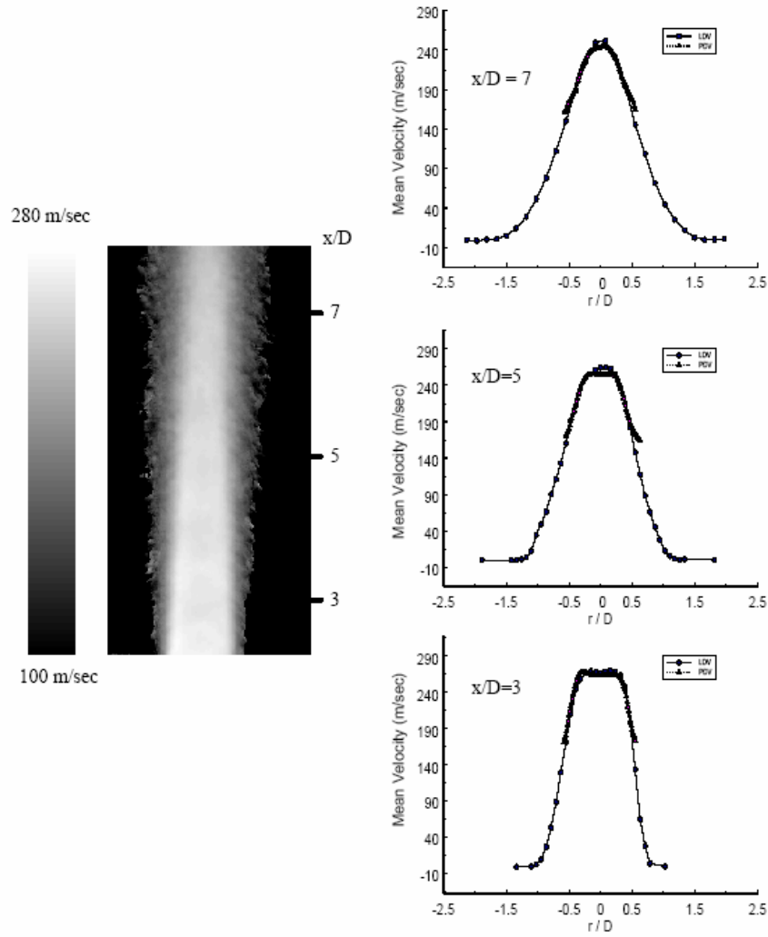
Figure 5.5 Average velocity measured in the Mach 1.36 Jet with PDV and comparison with LDV measurements at three streamwise locations. The direction of PDV sensitivity is 0.697i+0.123j-0.707 .
