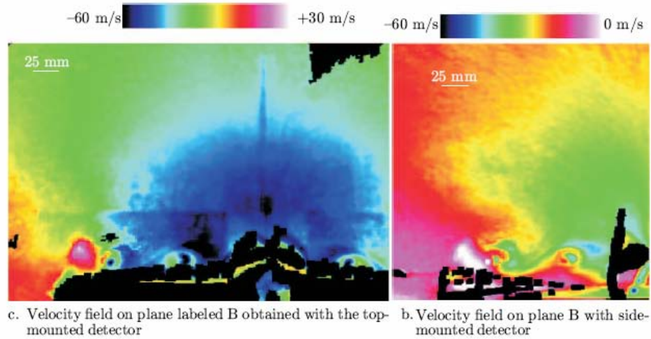
Figure 5.42 PDV velocity field of 56° delta wing model at 23° angle of attack in a Mach 0.2 free stream measured at plane B (trailing edge of canopy) with top- mounted (-0.253i, 0.0 j, 0.968k ) and side-mounted (-0.296i,0.421j,0.857k) cameras.
