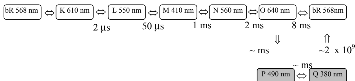
Figure 1. Photocycles of wild type bacteriorhodopsin at 292K and pH 7.
