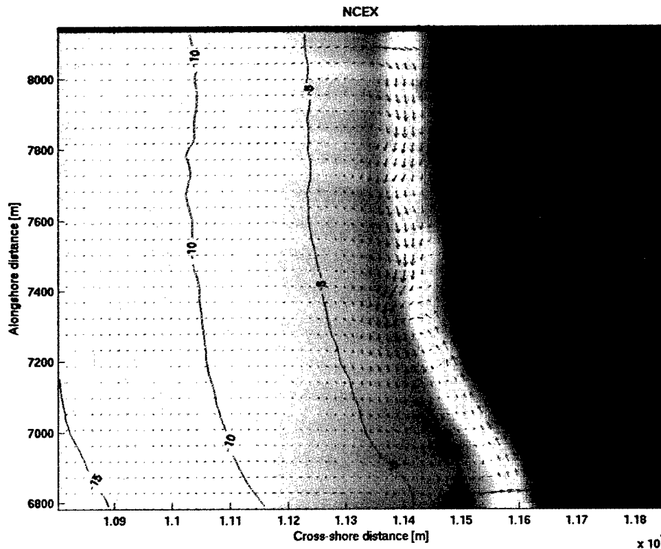
Figure 2 – Example nowcast product showing wave height and current patters for a 1.2 x 1.2 km nearshore region. Depth contours are in meters.
