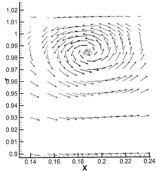
(b) Fine grid with MUSCL
