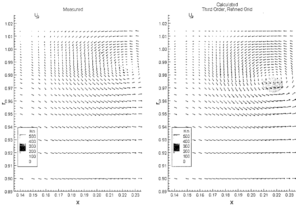
Figure 12: Computed and measured tangential velocity vectors and steamwise vorticity contours at s/C=0.4006 .
