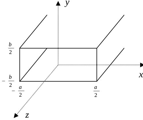
Figure 2-1. Geometry of a rectangular waveguide with the origin placed in the cross-sectional center.
