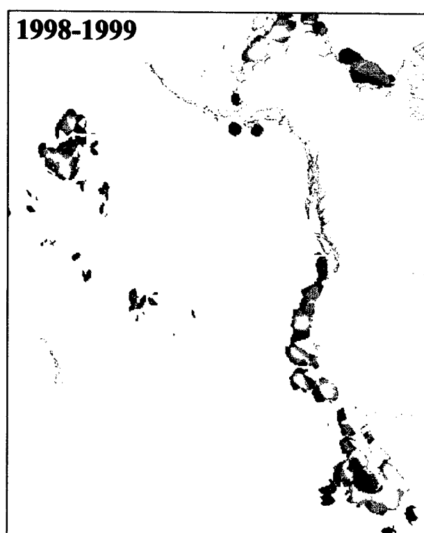
Figure 2. Persistence, in months per year, for concentrations of sea surface temperature fronts in the Northeast Pacific. Red values indicate exceptional densities of temperature gradients: 12 months per year. Green values indicate seasonal concentrations. The years defined June 1997-1998 (El Niño) and June 1998-1999 (La Niña) vary most in intensity near Baja California Sur and the North Pacific Transition Zone.
