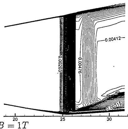
Fig. 4 Ionization degree in the vicinity of the ramp.
