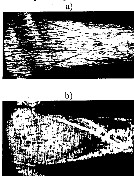
Рис.5. Shlieren pictures of flow at the interaction in a bulk of the diffuser except inlet part of diffuser. a) V=110V , B=0 , б) V=110V , B=1.3T
