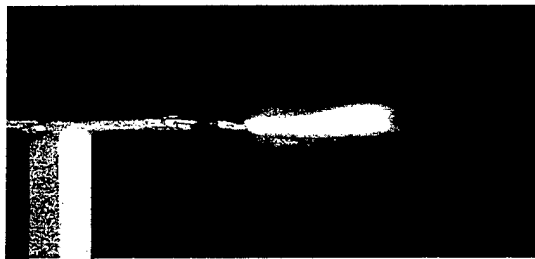
Fig.2 Deeply undercritical microwave discharge in SS flow, M = 2 , P = 2,1 kW
