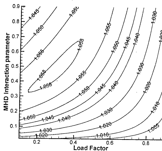
Fig.7 Contours of relative specific impulse for scramjet with MHD control with \theta_N=15^\circ , M_d=10 , F_{ih}=0.12 , M_0=6 , q/q_{cr}=0.01 .
