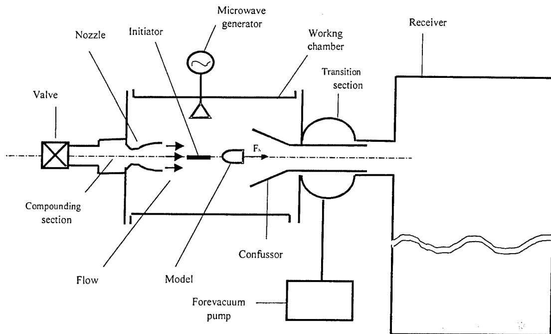
Fig.1. A scheme of experimental set up.
