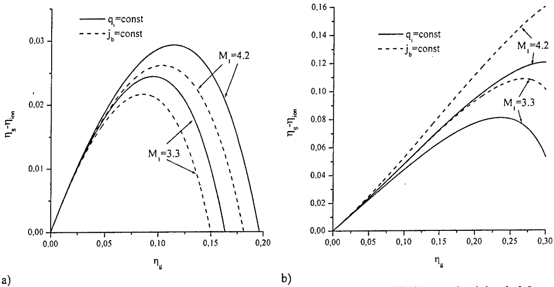
a) b) Fig.3 Relative power excess produced by Faraday MHD generator with nonequilibrium conductivity: k=0.5 , q_i=\text{const} for solid lines j_b=\text{const} for dashed lines. Mach number at MHD generator entrance is shown near the curves, q_i/q_{cr}=0.3 . a) \xi = \tilde{\xi} , b) \xi=0
