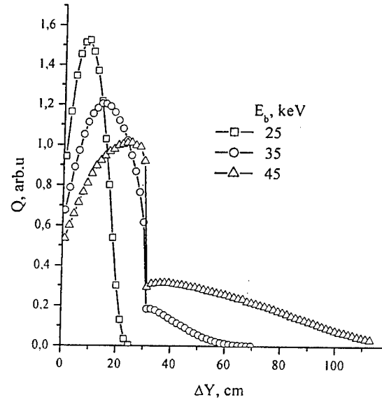
Fig.10 E-beam power deposition profile in flow over the wedge ( 10^\circ ). E-beam is located at x=3\text{m} (Fig.7), initial energies in e-beam are shown in the figure.
