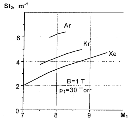
Fig. 4 The values of the initial local Stewart parameter versus the Mach numbers of the incident shock wave for various gases.
