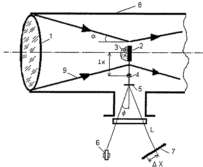
Fig.1. Scheme of modeling experiment 1 – lens forming of convergent microwave beam; 2 – metal-dielectric target; 3 – plasma of non-self-sustained microwave discharge; 4 – pendulum; 5 – mirror; 6 – laser; 7 – screen; 8 – vacuum chamber; 9 – convergent microwave beam
