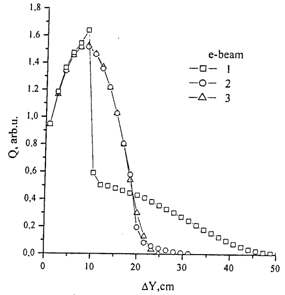
Fig.8 E-beam power deposition profile in flow over the wedge ( 10^\circ ). Positions of e-beam correspond to the Fig.7.
