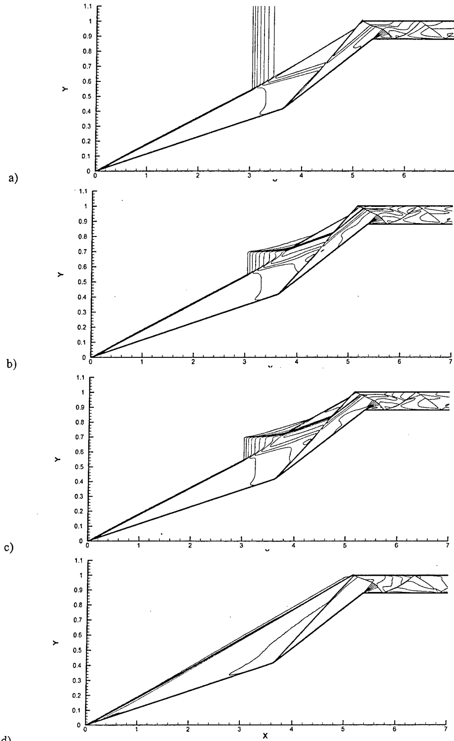
d) Fig.2. Mach number contours in MHD controlled inlet. M_0=12 , M_\infty=10 , B=1\text{T} , k=0.5 . Ionized region a) 3 \leq x \leq 3.5 ; b) and c) 3 \leq x \leq 4 , Y \leq 0.7 ; d) 0 \leq x \leq 5 , Y \leq 0.2x ; \alpha=90^\circ in (a,b), \alpha=45^\circ in (c,d); q_i [\text{W}/\text{cm}^3] =a) 0.2, b) 0.2, c) 4.5, d) 1.2.
