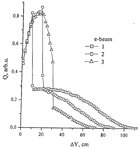
Fig.9 E-beam power deposition profile in flow over the wedge ( 10^\circ ). Positions of e-beam correspond to the Fig.7.
