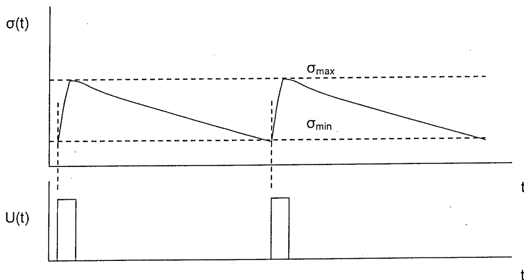
Fig.3. An action of the inhibitor of the plasma decay in impulse - periodic operational mode of the energization source.
