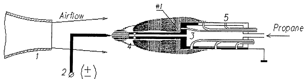
Fig.1 . Scheme of experimental setup (variant-2):
