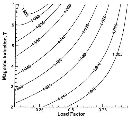
a) b) Fig.9 Contours of relative specific impulse (a) and power excess (b) for scramjet with MHD control with \theta_N=15^\circ , M_d=10 , F_{th}=0.12 , M_0=6 , L=2m , k_3=1.1 , q_i=1W/cm^3
