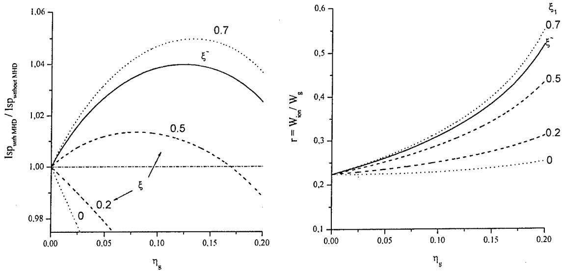
a) b) Fig.4 Relative specific impulse (a) and relative power spent on ionization (b) for MHD generator with various parameters \xi_i . \theta_N=15^\circ , M_d=10 , F_{th}=0.12 , M_0=6 , q_i/q_{cr}=0.05 , power density q_i is constant in MHD generator volume.
