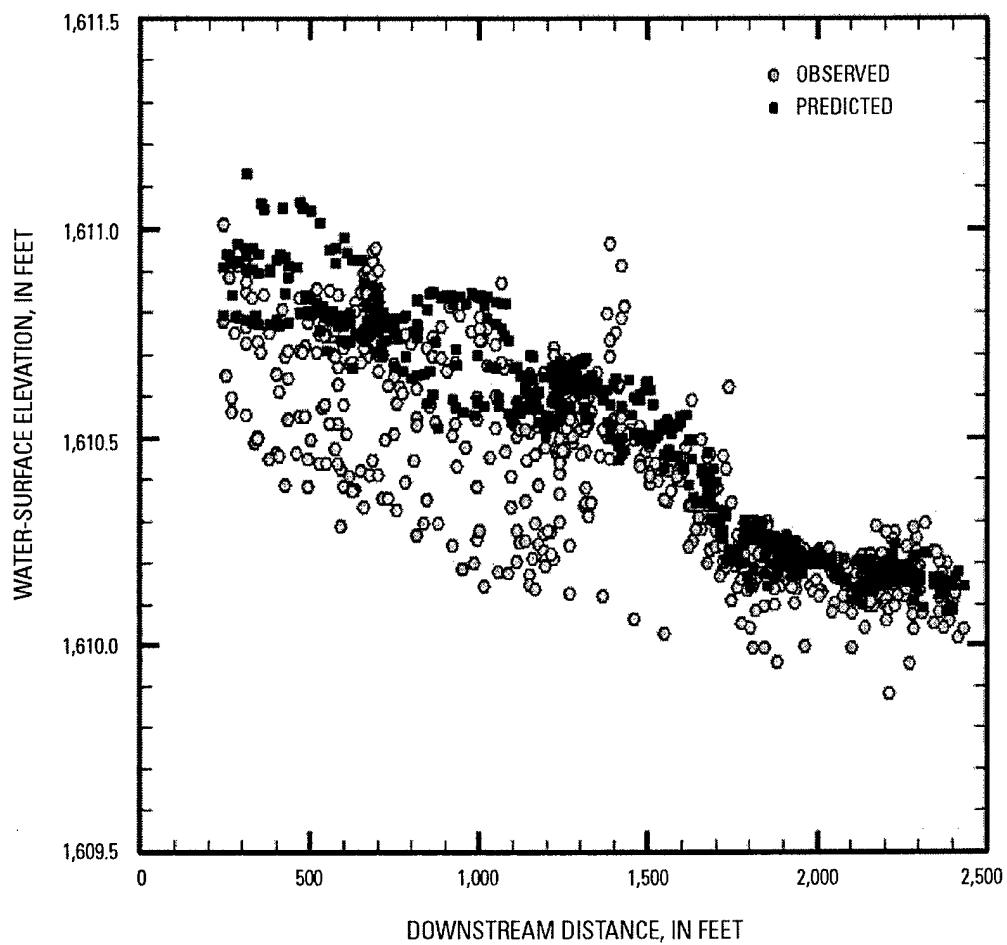
Figure 3. Predicted and observed values for water-surface elevation for the calibration discharge of 25,600 \text{ ft}^3/\text{s} at bridge 505 of the Alaska Highway over the Tanana River near Tok, Alaska.
