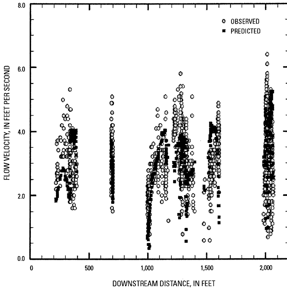
Figure 4. Predicted and observed values for water velocity for the calibration discharge of 25,600 ft 3 /s at bridge 505 of the Alaska Highway over the Tanana River near Tok, Alaska. The distribution of points in the vertical direction represents the variation in velocity magnitude across the channel.
