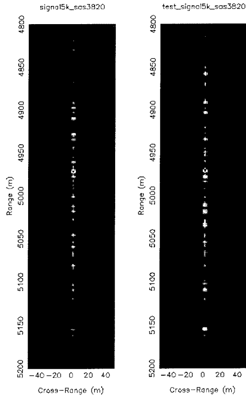
Figure 2-30. Salmon SAS simulation single point at 5 km, flat bottom. Left image uses SVP from Figure 2-22. Right image uses constant SVP.
