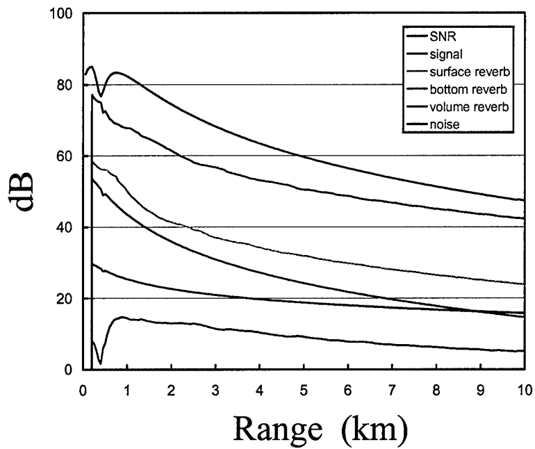
Figure B-3. Simulation results: deep water, coarse sand bottom, directional transmission mode, 2 second chirp.
