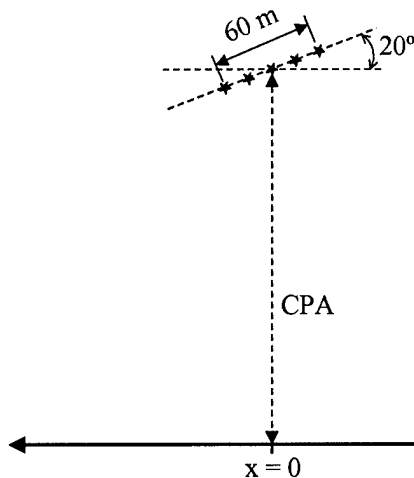
Figure 2-15. Five-point target configuration.
