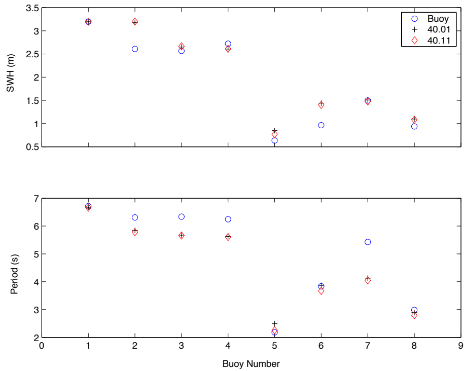
Fig. 3 — SWAN output and buoy data comparisons for significant wave height and mean wave period for Test 1, Case 2, which represents wind speed and direction at 12 m/s and 300 deg on 10/14/82 at 22.00 h UTC
