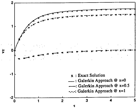
Fig. 10 Time response, P = \Phi_1^0 , \chi = 0^\circ , z=0, y=0 .
