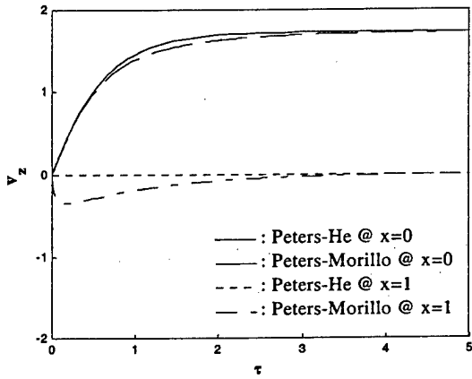
Fig. 11 Time response, P = \Phi_1^0 , \chi = 0^\circ , z=0, y=0 .
