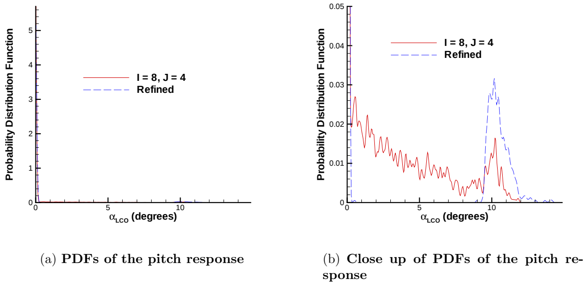
Figure 5.12 Convergence of the pitch subcritical response
