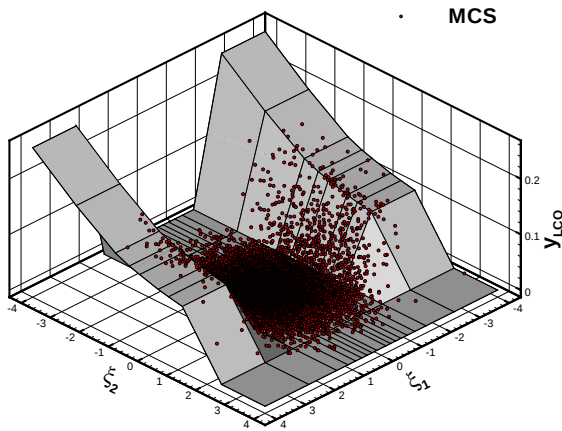
(a) B-spline surface from the Gaussian nodes ( I = 8, J = 4 )
