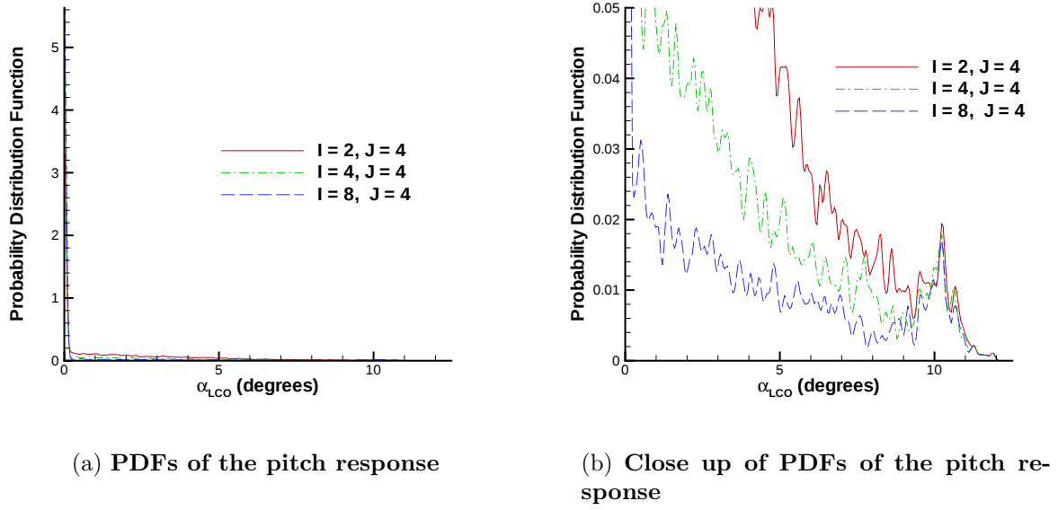
Figure 5.9 Pitch Response
