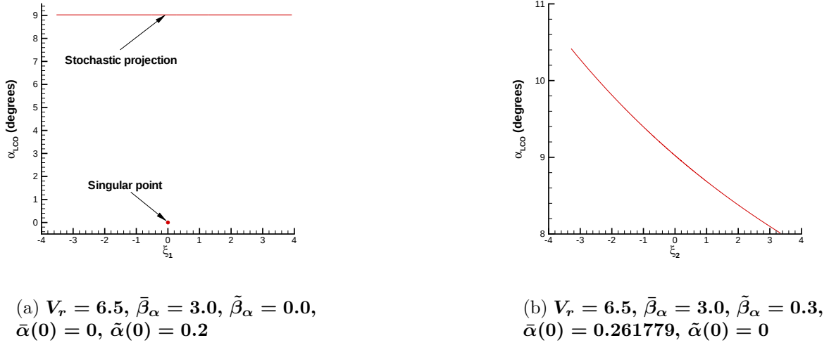
Figure 3.1 Stochastic projection of \alpha_{LCO} onto the random variables \xi_1 and \xi_2 (super-critical response)
