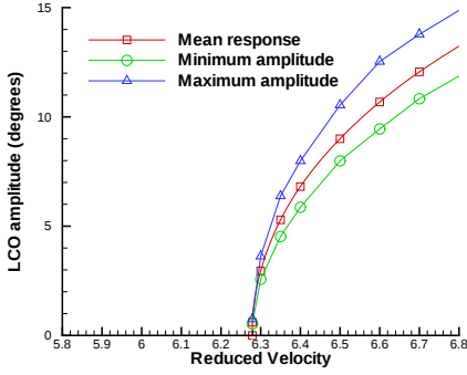
(a) Supercritical response
