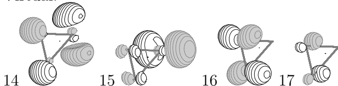
Figure 37 Valence Orbitals for Triangular X 1 \Sigma SiC 2
