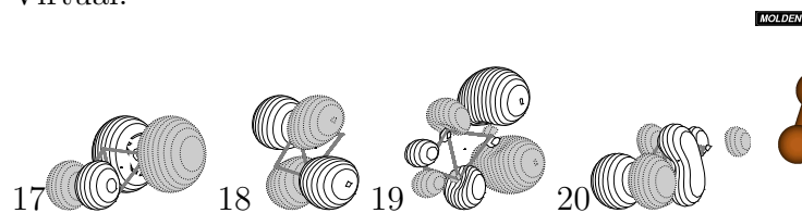
Figure 33 Valence Orbitals for C-C Bonded Rhomboidal X ^1A_1 SiC 3
