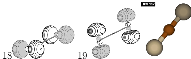
Figure 17 Valence Orbitals for Linear X ^1\Sigma Si 2 C
