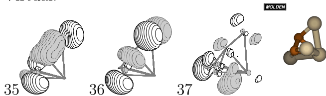
Figure 42 Valence Orbitals for Distorted C_{1v} ^1A_1 Si_4C_2
