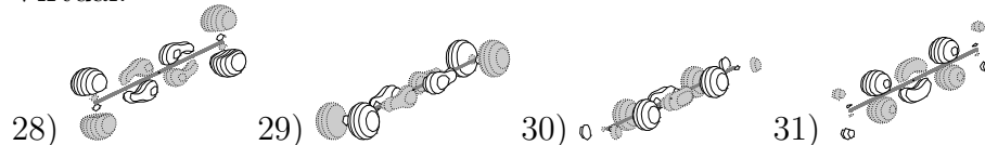
Figure 26 Valence Orbitals for Linear X 1 Σ Si 2 C 4
