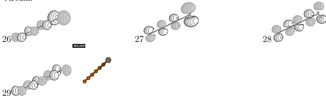
Figure 21 Valence Orbitals for Linear X \ ^1\Sigma \text{SiC}_6
