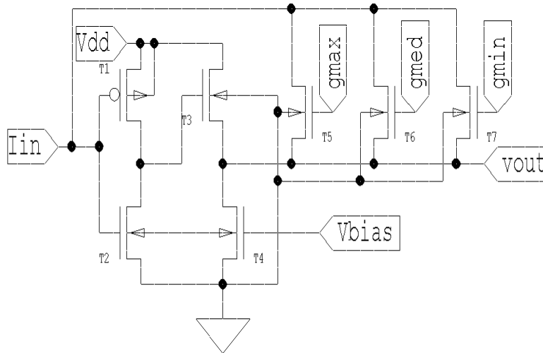
Figure 6-10. Transimpedance amplifier
