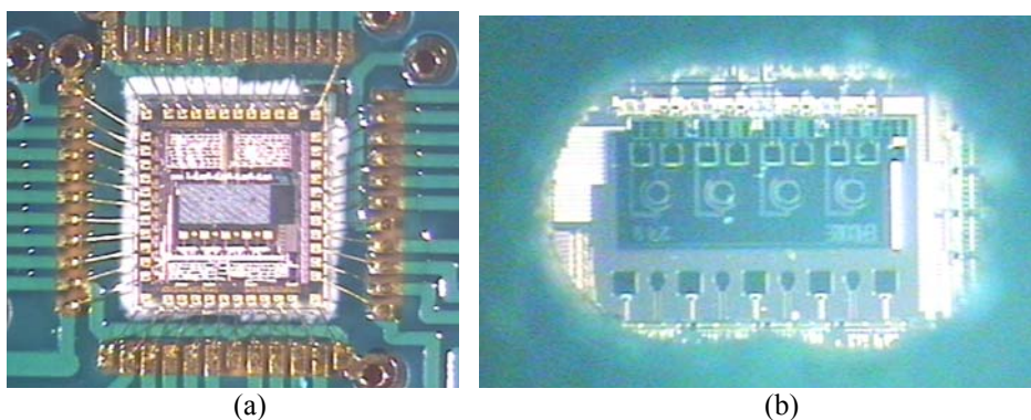
Figure 6-13. Chip-on-board (a) Front view (b) Back view
