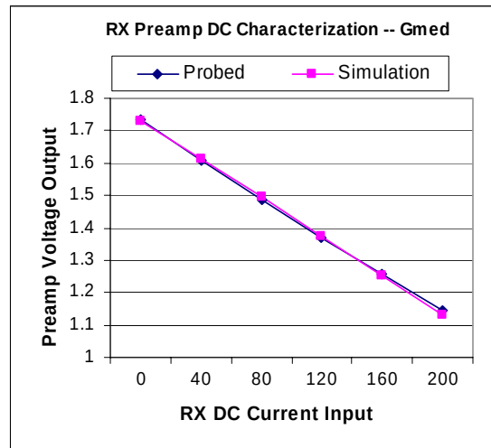
Figure 6-11. Receiver pre-amplifier DC output comparison between simulation and test result
