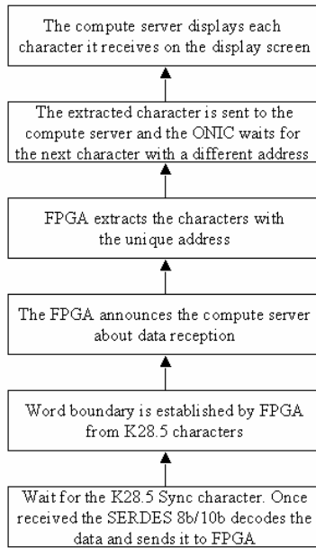
Figure 2-8. Message passing application test sequence
