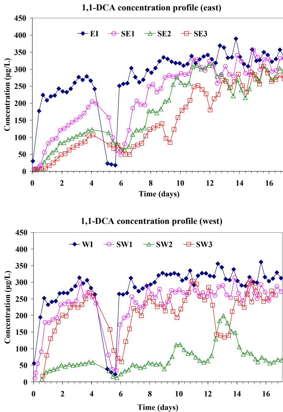
Figure 5.5 1,1-DCA concentrations in the injection wells and the monitoring wells in the two test zones (east, bioaugmented; west, non-bioaugmented) at Moffett Field (data from Gary Hopkins at Stanford University, CA)
