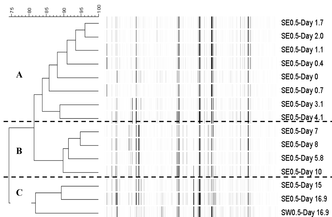
Figure 5.11 A GelCompar II-generated UPGMA clustering dendrogram and corresponding normalized restriction profiles from the community DNA extracted from the bioaugmentation experiment samples in well SE 0.5 and SW0.5.
