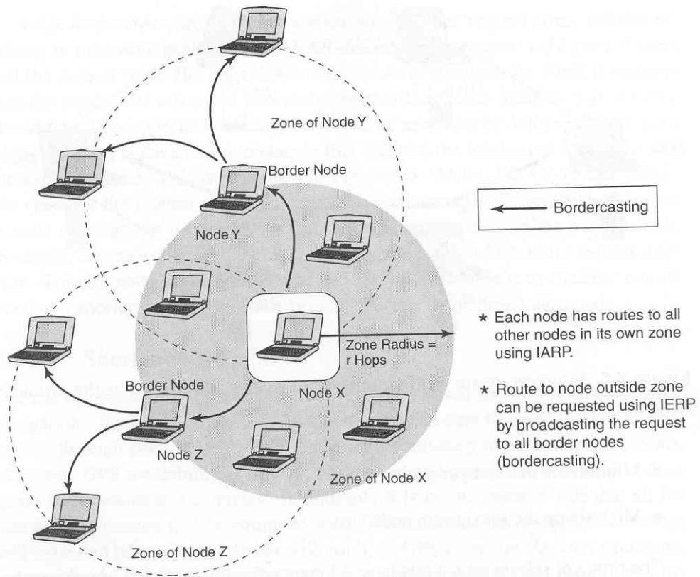
Figure 19. Hybrid approach – ZRP (From [2]).
