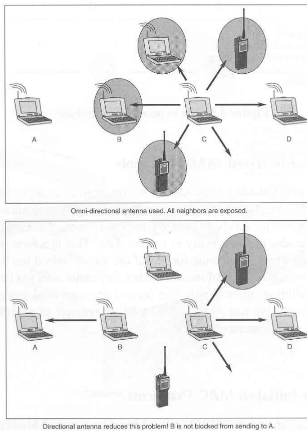
Figure 6. Solution of Exposed Node Problem by Unidirectional Antennae (From [2]).
