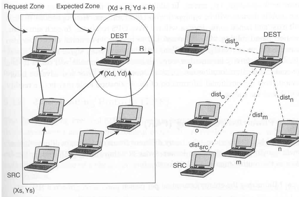
Figure 17. (a) Concept of request zone and expected zone in LAR (b) Consideration of route physical distance (From [2]).
