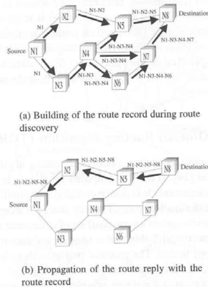
Figure 15. DSR source route creation process (From [2]).
