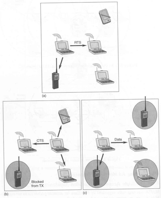
Figure 7. Controlled Handshake used in CSMA-CA (From [2]).
