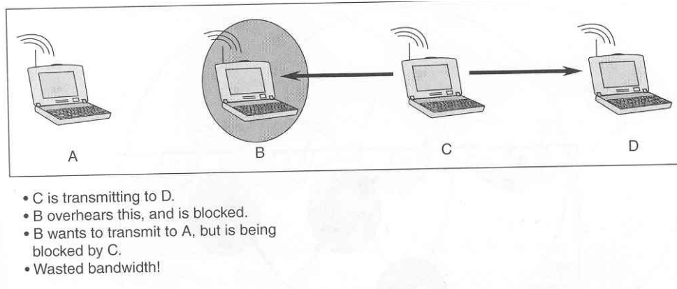
Figure 5. Exposed Node Problem (From [2]).
