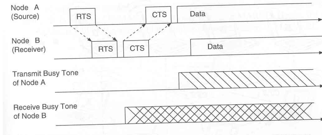
Figure 10. DBTMA Principle (From [2]).
