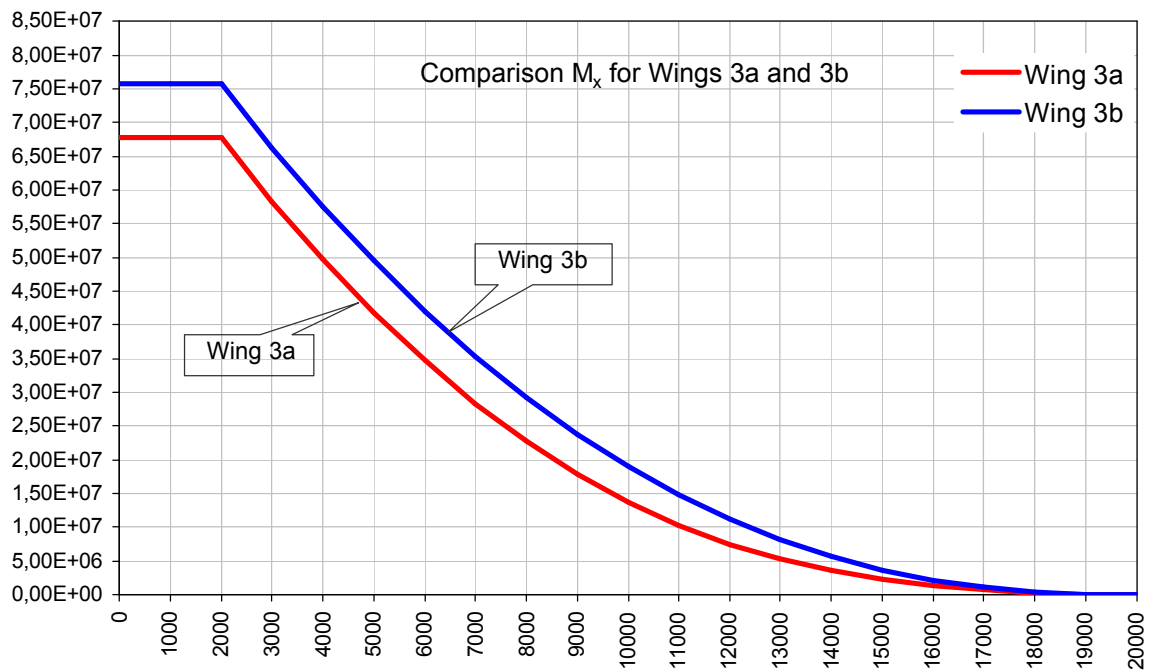
Figure 9.16 – Comparison M_x for wings 3a and 3b
