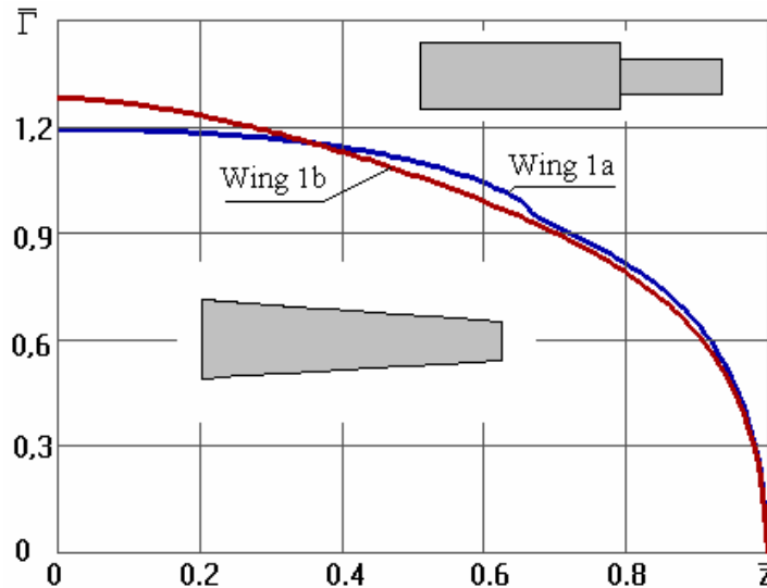
Figure 9.8 – Wings 1a, 1b dimensionless velocity circulation
