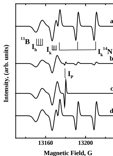
Fig.3.1.4. Photoresponse of EPR spectra in s.-i. 4H-SiC measured at 77 K and \mathbf{B} \perp \mathbf{c} . a: UV light excitation, b: Spectra 21 hours after UV illumination, c: Visible light excitation, d: UV quenching of visible light induced signal.
