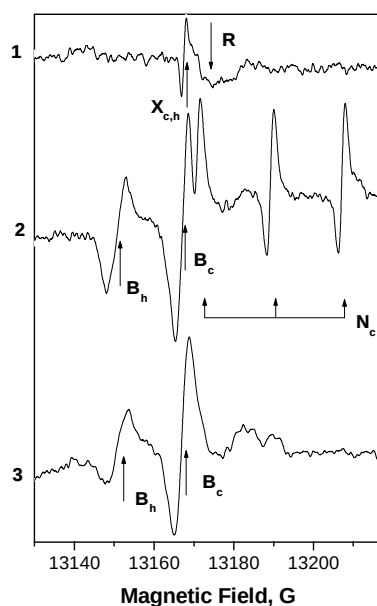
Fig. 4.1.3. Photoresponse of EPR spectra in (D4) F0847 s.-i. sample measured at 37 GHz and 77 K. 1 – dark; 2 – illumination with UV light; 3 - 26 h after the light is switched off. \mathbf{B}_0 \perp \mathbf{c} . \mathbf{B}_c , \mathbf{B}_h -EPR spectrum of boron ^{11}\text{B} , \mathbf{N}_c - EPR spectrum of nitrogen.
