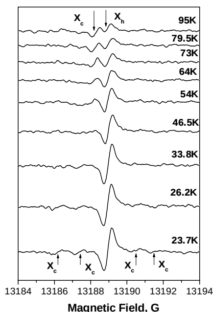
Fig. 4.1.1. Temperature transformation of X defect EPR spectrum.
