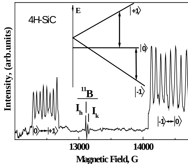
Fig. 1.4.1. Vanadium V^{3+}(3d^2) EPR spectrum in s.-i. 4H-SiC measured at T = 4.2 K, 37 GHz and \mathbf{B} \parallel \mathbf{c} . The two hyperfine octets belong to the V^{3+}(3d^2) cubic site. The energy level scheme for a triplet system in a static magnetic field is shown for D > 0 .
