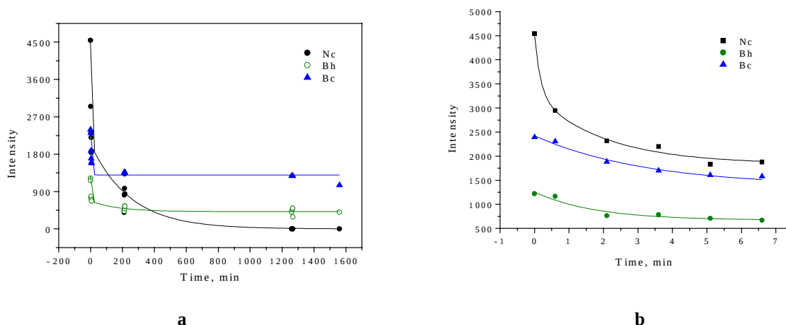
Fig.3.1.5. Decay of nitrogen and boron EPR line intensity after UV excitation light (band gap) is switched off - a . Fast component of decay curve of the carrier concentration captured by nitrogen and boron energy levels - b . T = 77 K. Sample F0847
