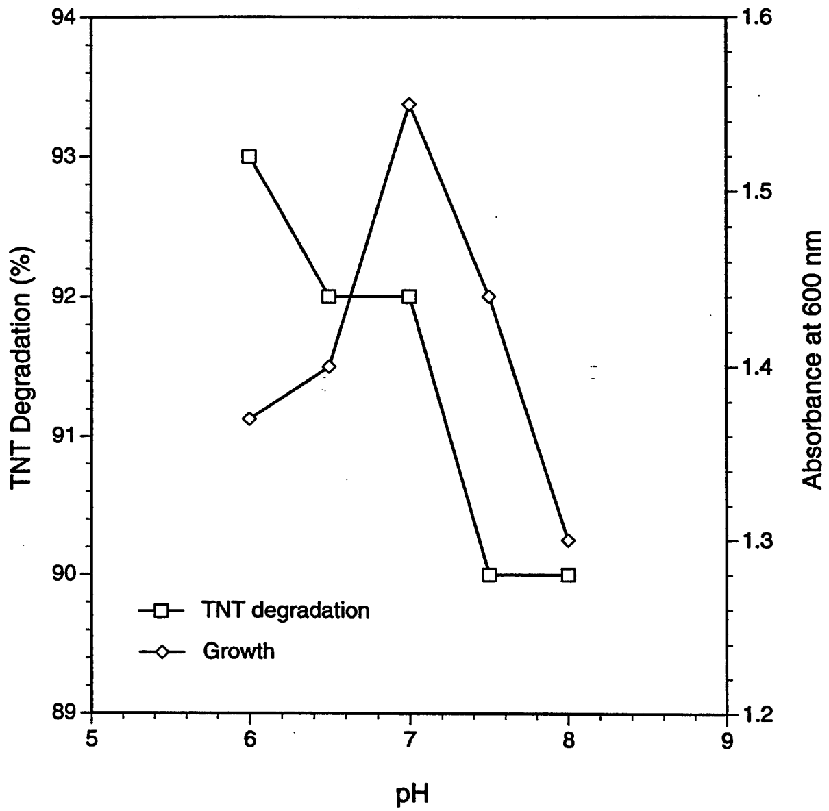
FIGURE 14 Effect of pH on TNT Metabolism
