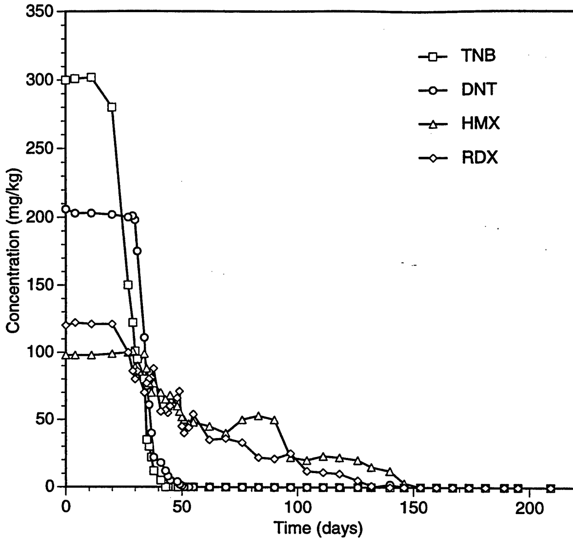
FIGURE 34 Concentrations of Munitions Compounds in the Reactor
