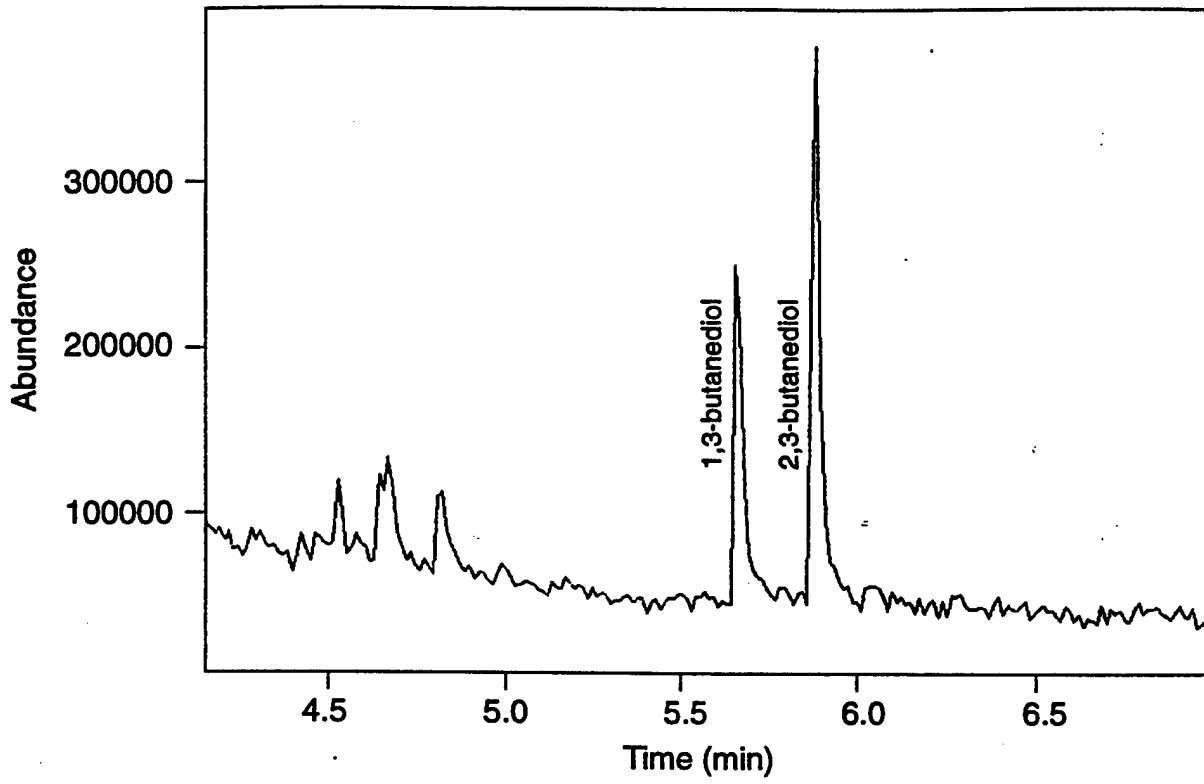
FIGURE 41 GC/MS Chromatogram of 2-min HPLC Peak in Figure 40
