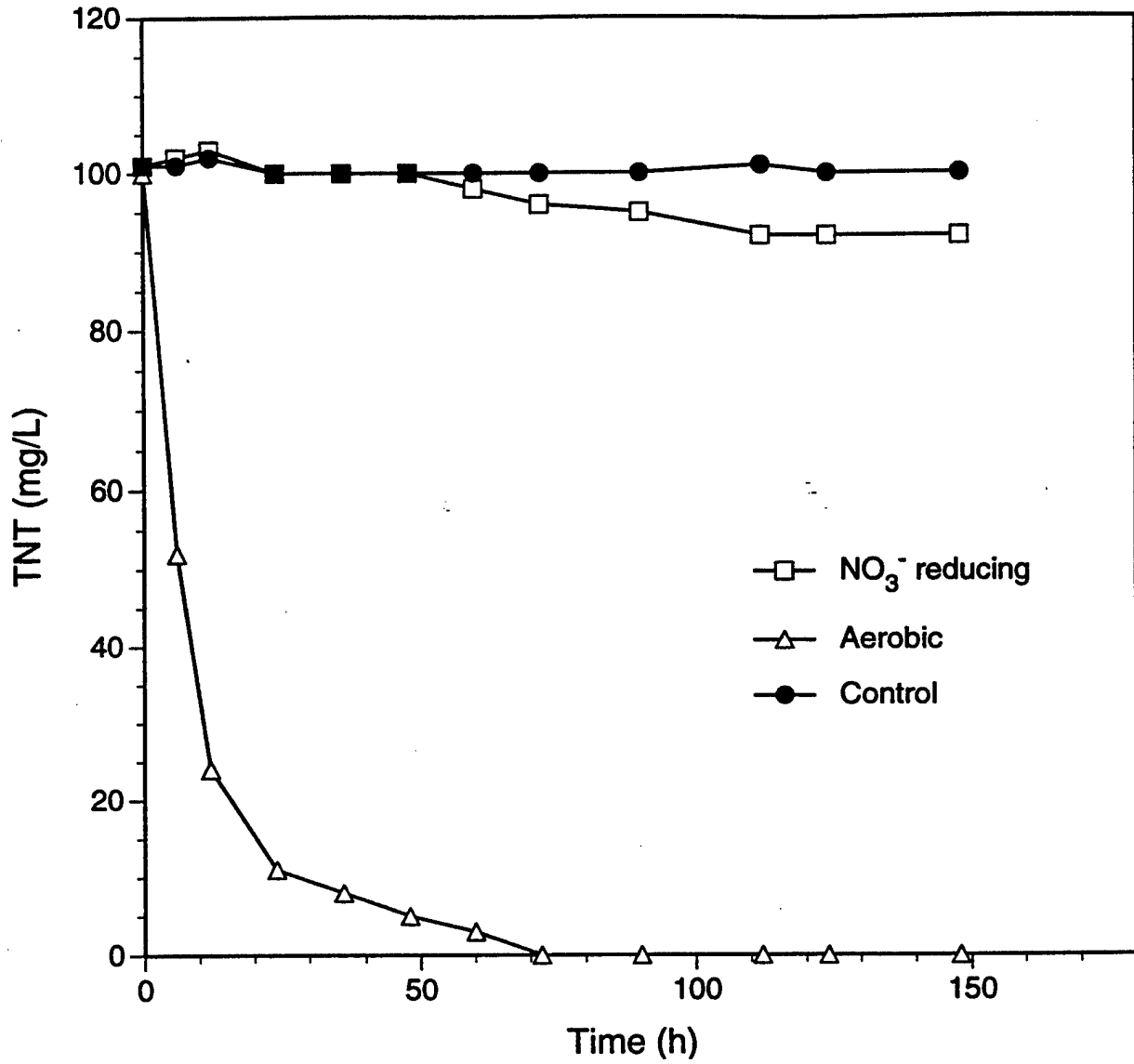
FIGURE 18 TNT Metabolism under Aerobic and Nitrate-Reducing Conditions
