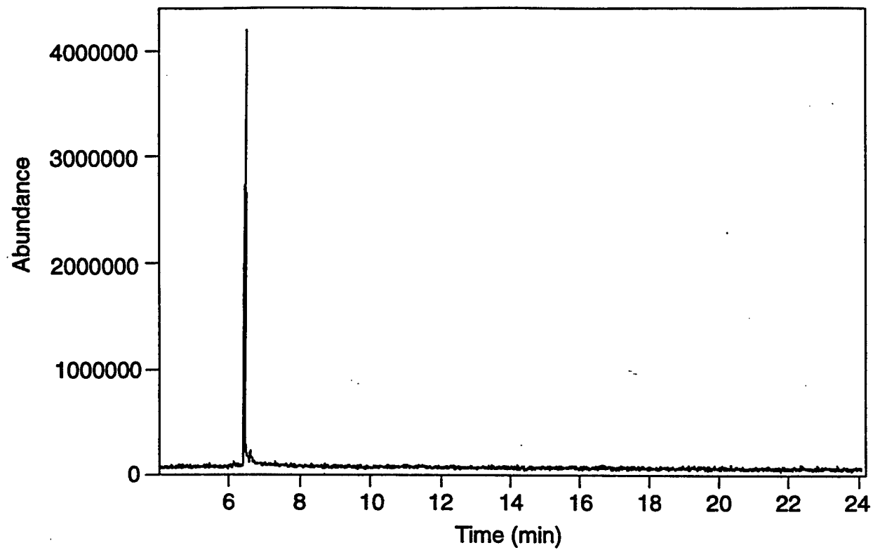
FIGURE 43 GC/MS Chromatogram of 2,3-Butanediol Standard
