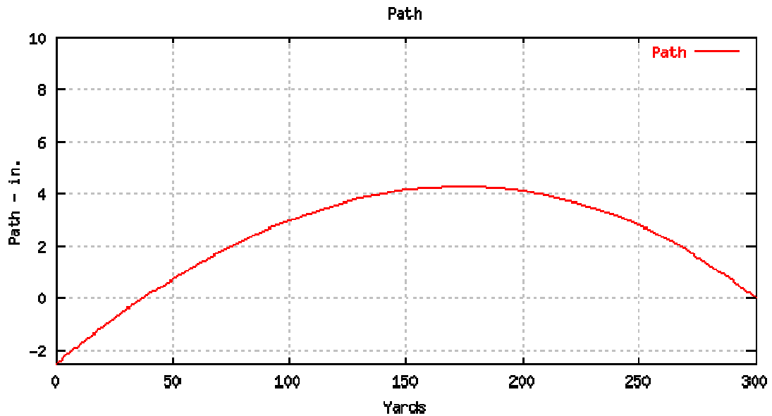
Figure 16. Trajectory of M855 Ammunition at 300 Yard Zero
