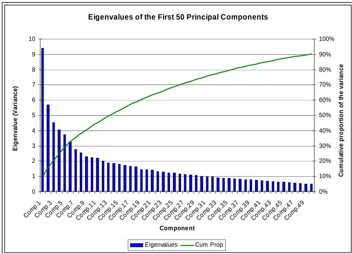
Figure 30. Eigenvalues of the first 50 principal components with corresponding cumulative proportion of the total variance explained by the eigenvalues.
