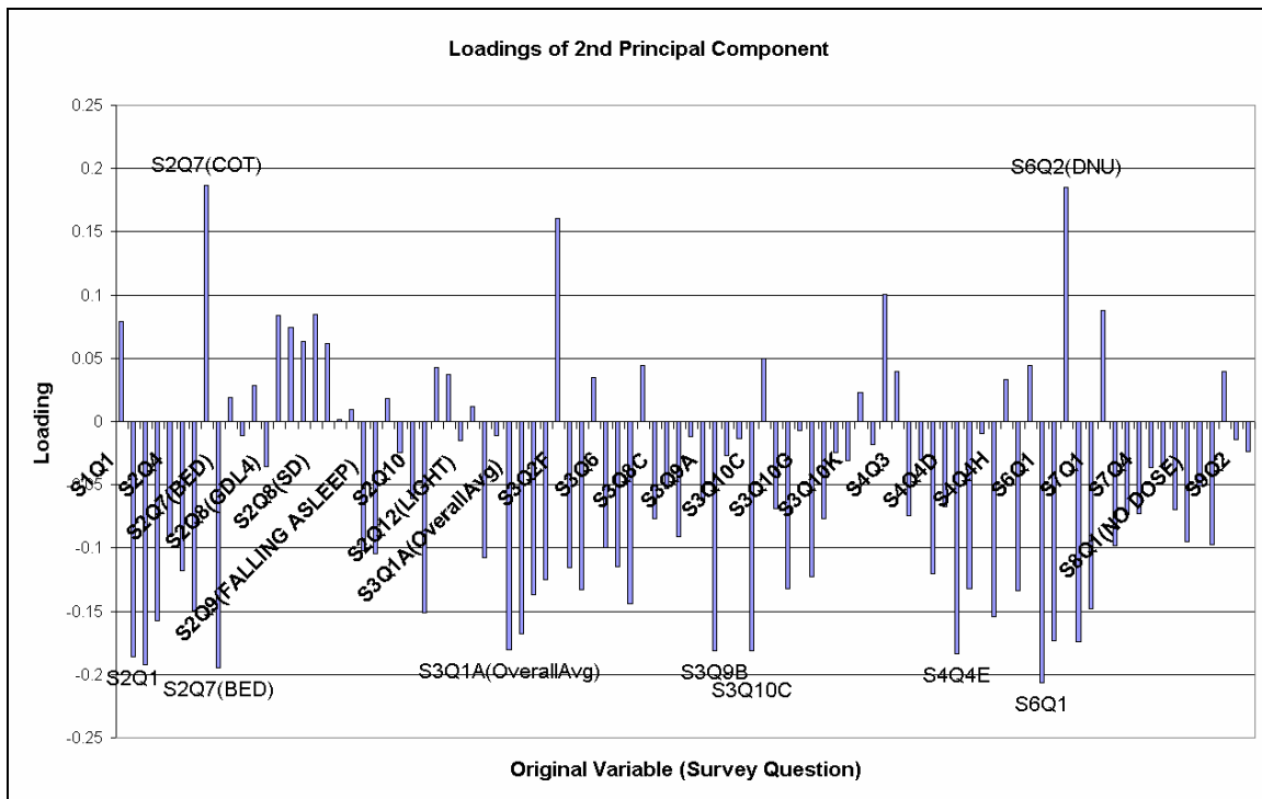
Figure 32. Loadings of the second principal component.
