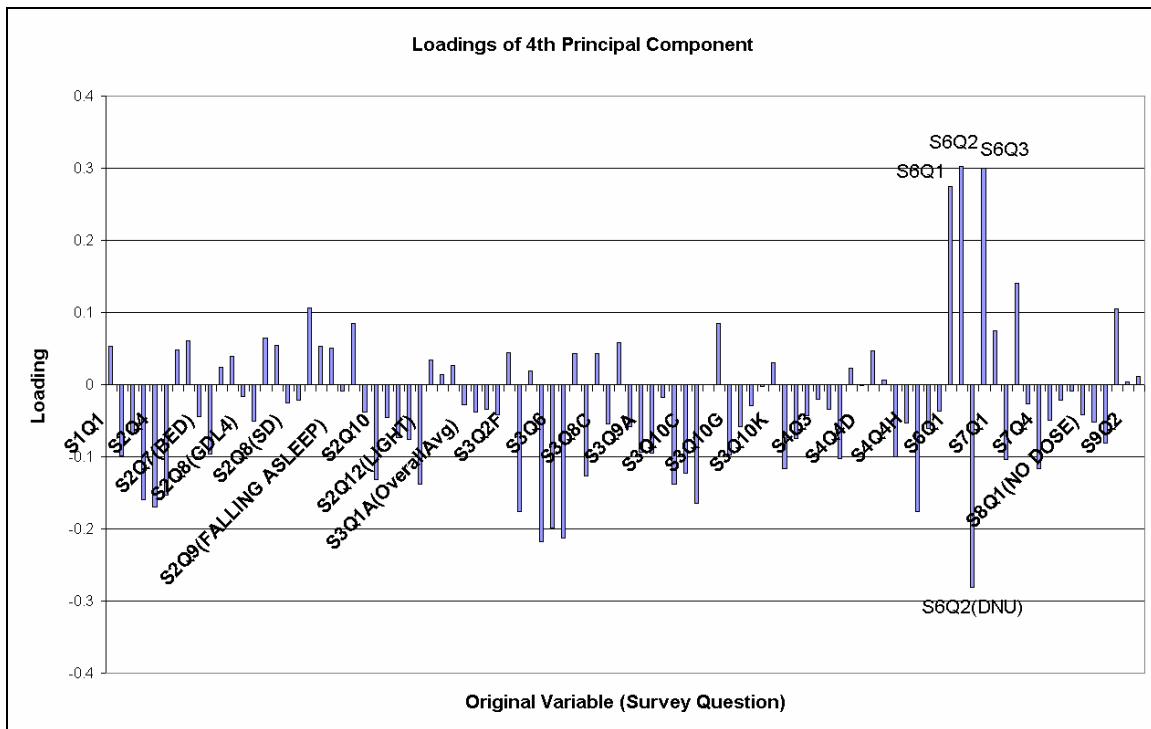
Figure 34. Loadings of the fourth principal component.
