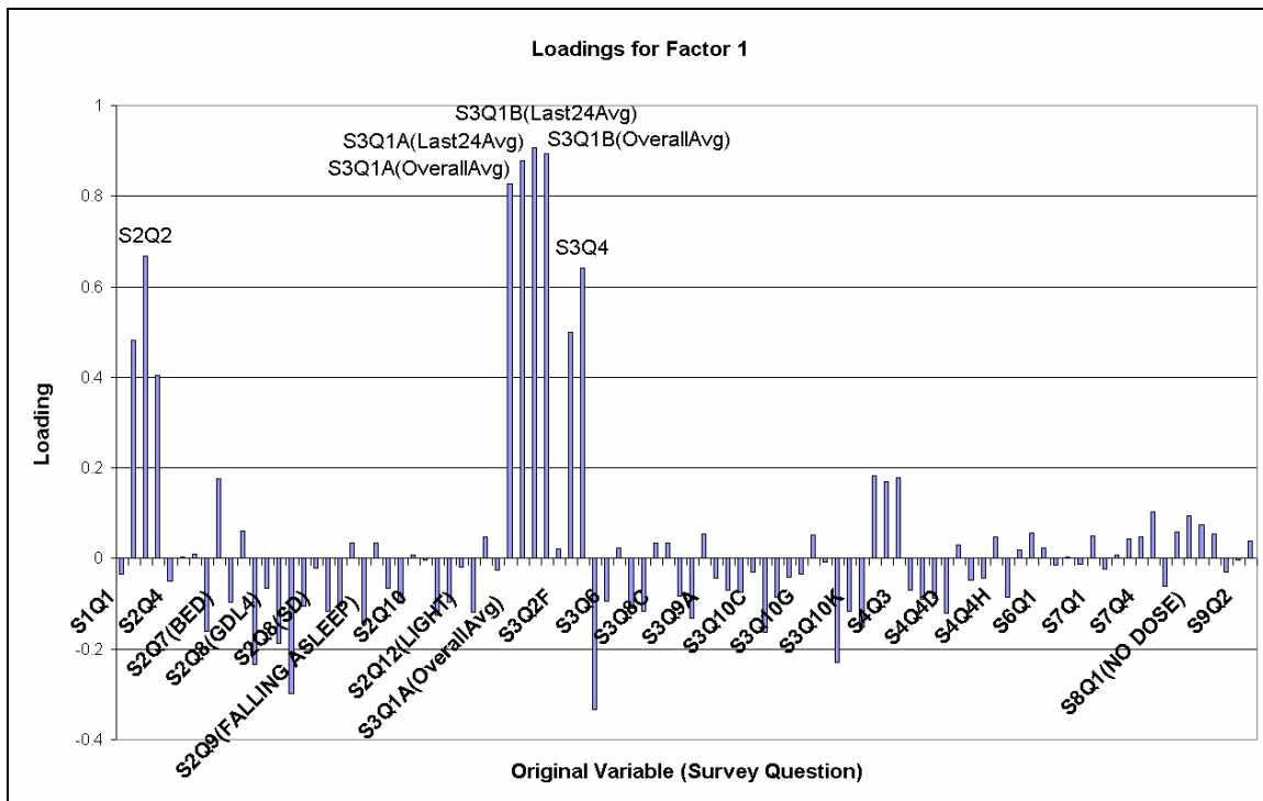
Figure 36. Loadings for the first factor.
