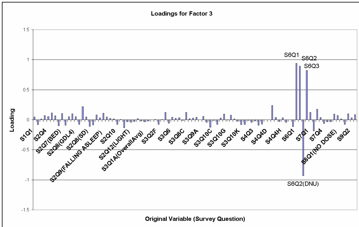
Figure 38. Loadings for the third factor.
