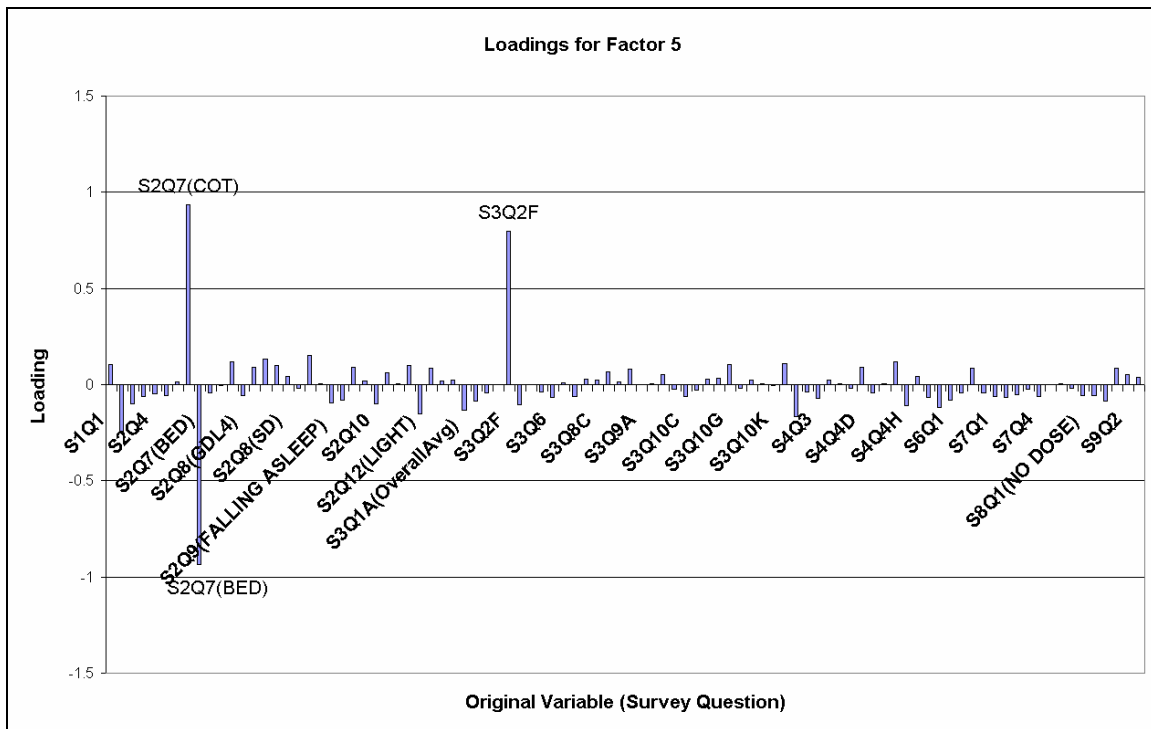
Figure 40. Loadings for the fifth factor.
