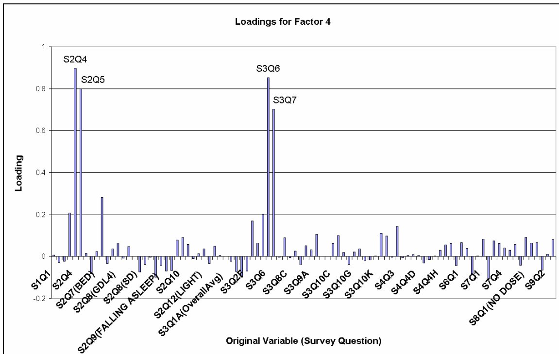
Figure 39. Loadings for the fourth factor.
