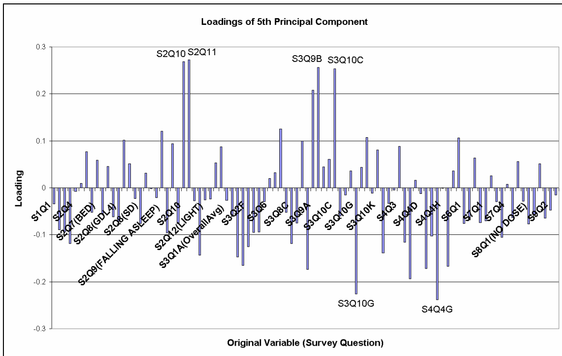
Figure 35. Loadings of the fifth principal component.
