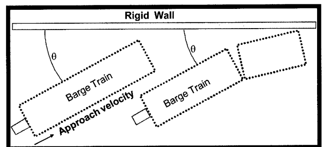
Transverse Failure
