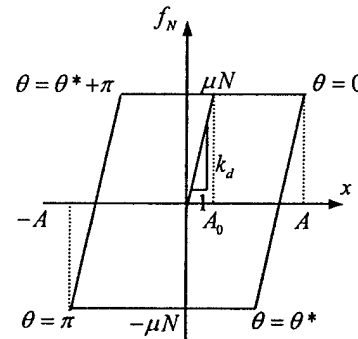
Figure 2: Hysteresis from spring damper element
