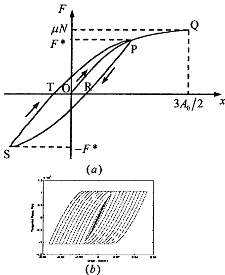
Figure 14: Hysteresis from Mindlin analysis
