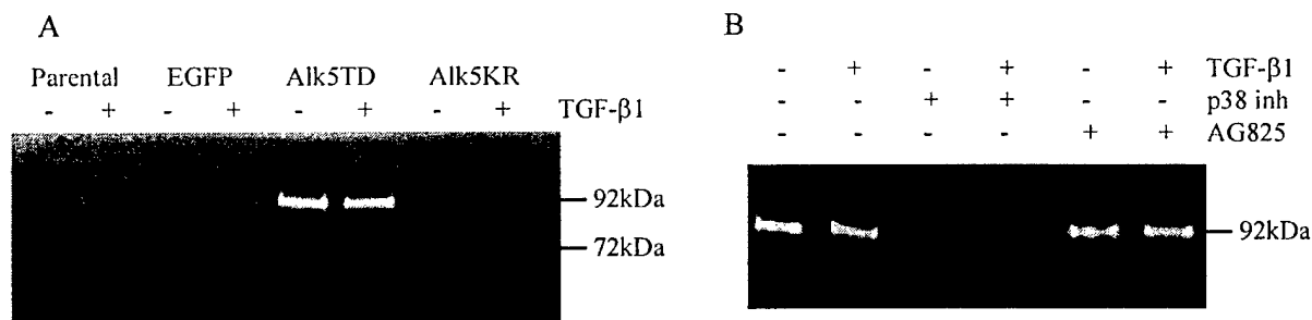
Fig.6. Gelatin gel zymography assay in MDA-MB-231 cells. Where it is indicated cells were treated with 2ng/ml TGF- \beta 1 and 10 \mu M p38 inhibitor, or 5 \mu M AG825, a Neu/Erb-B2 inhibitor.
