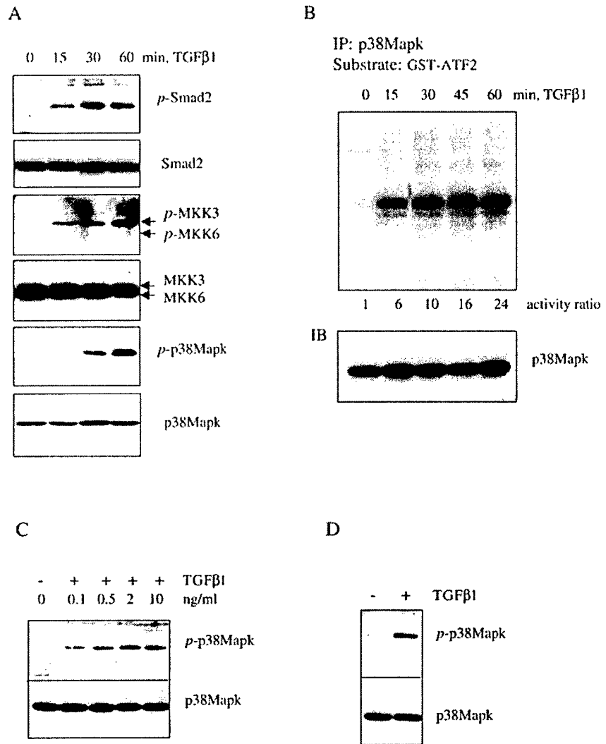
Fig. 3. Activation of the p38MAPK pathway in response to TGFβ. NMuMG cells were incubated in serum-free medium for 4 hours before addition of TGFβ1. (A) Immunoblot analyses with antibodies to phospho-Smad2, phospho-MKK3/6 and phospho-p38MAPK, and total Smad2, MKK3/6 and p38MAPK. (B) Detection of p38MAPK kinase activity in whole-cell extracts from NMuMG cells treated with 2 ng/ml TGFβ1 using GST-ATF2 as substrate. The products were separated by SDS-PAGE and transferred onto nitrocellulose-membrane. 32 P incorporation into ATF2 was quantitated using PhosphorImager. The membrane was probed with antibody to p38MAPK. (C) Immunoblot detection of TGFβ1 dose-dependent effect on p38MAPK phosphorylation at 60 minutes in NMuMG cells. (D) Induction of p38MAPK phosphorylation by 2 ng/ml TGFβ1 at 60 minutes in SiHa cells.
