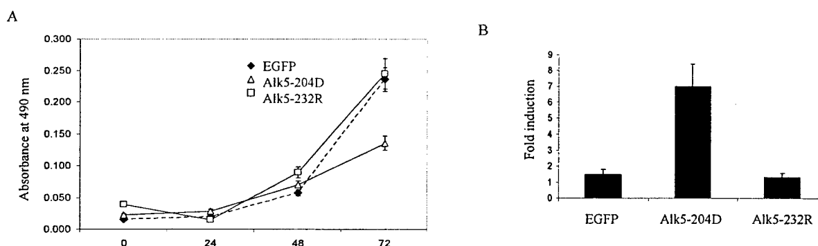
Fig.5. Alk5-204D reduces cell proliferation but stimulates invasion of MDA-MB-231 cells.
