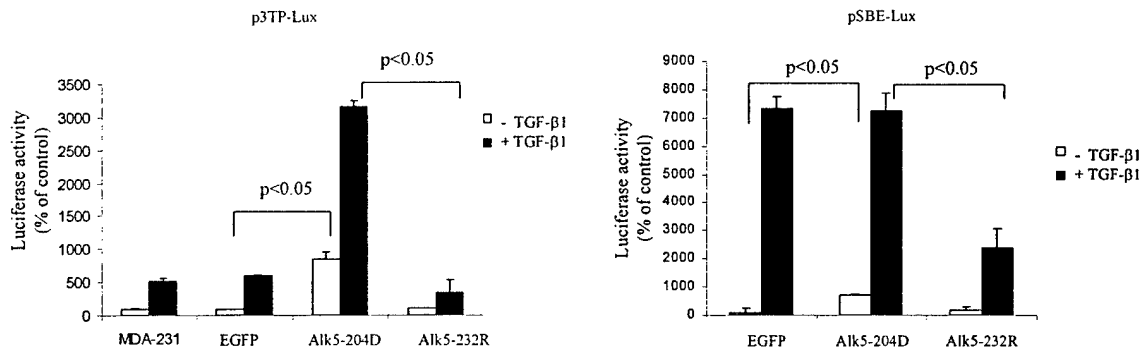
Fig. 2. Luciferase reporter activity in parental and genetically engineered MDA-MB-231 cells (see text) co-transfected with the p3TP-Lux reporter (left panel), or pSBE-Lux (right panel) pCMV-Renilla. Firefly and Renilla luciferase activities were measured using Promega's dual luciferase reporter assay system. Each data point represents the mean ± S.D. of three wells. p < 0.05 compared to control using ANOVA test.
