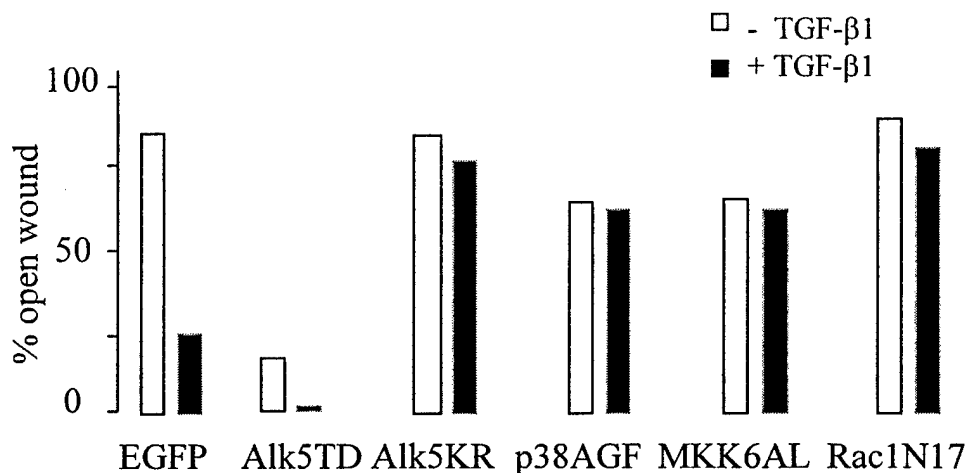
Fig.7. Dominant-negative mutants of the p38 MAPK pathway inhibit TGF \beta -mediated cell motility in MDA-MB-231 cells. Monolayers of MDA-MB-231 cells expressing EGFP only and various mutants were wounded with a plastic tip. Cells were incubated with 2 ng/ml TGF- \beta 1 where it is indicated. The graph shows the remaining wound area measured after 24h of incubation relative to the initial area.
