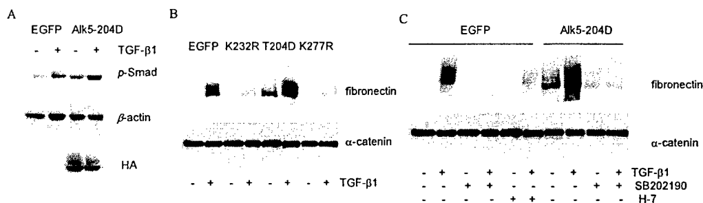
Fig. 1. Effect of kinase-mutants on phosphorylation of Smad2/3 (A) and expression of fibronectin in MDA-MB-231 cells treated with 2 ng/ml TGF- \beta 1, and 20 \mu M of H-7 or 10 \mu M SB202190.
