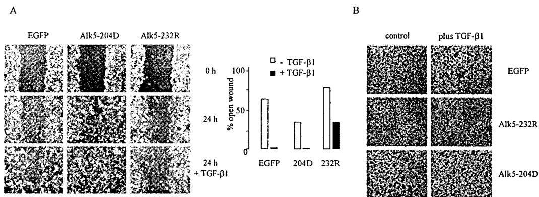
Fig. 3. Migration of MDA-MB-231 cells expressing TβRI/Alk5 kinase-mutants. (A) Wound closure in cell monolayers after 24 h of treatment with 2 ng/ml TGF-β1. Phase contrast images were recorded at 100x magnification. Similar results were obtained three times. (B) MDA-MB-231 cells ( 1 \times 10^5 /well) were seeded in the upper chamber of 5-μm pore transwells and incubated for 16 h with 2 ng/ml TGF-β1 added to the lower chamber. Cells migrated through pores were stained and counted from four random fields. Representative pictures are shown. Experiments were performed in duplicates.
