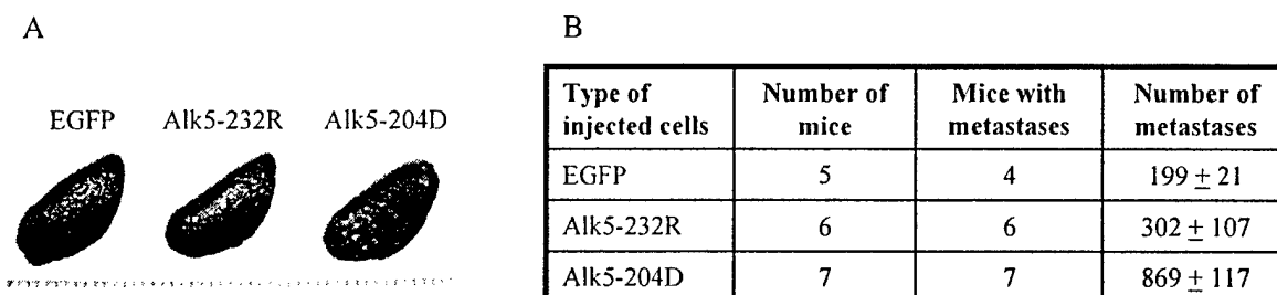
Fig.4. Alk5-204D increases formation of pulmonary macrometastatic lesions by MDA-MB-231 cells in SCID mice.
