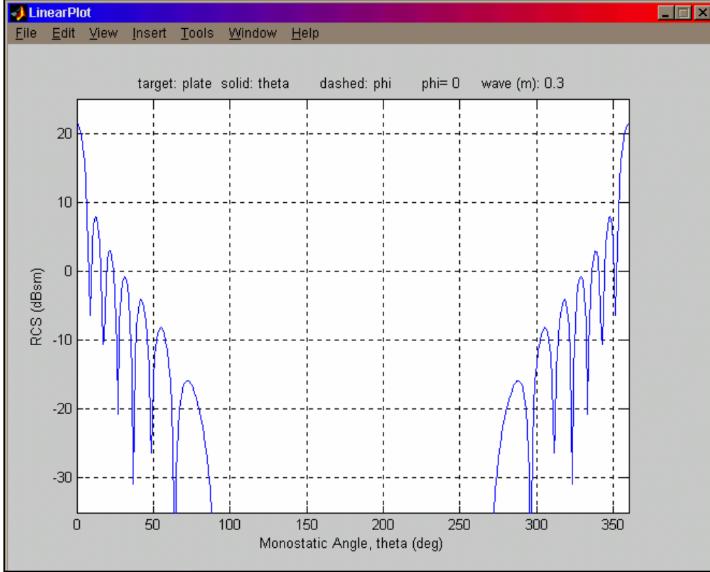
Figure 39. RCS of a 1 m by 1 m PEC Plate at 1 GHz, TM wave, for \mathbf{f}=0
