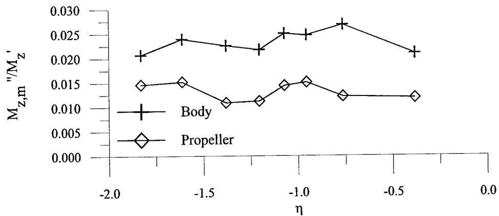
Figure 2.11 Standard deviation of mean M_z' as fraction of mean M_z'
