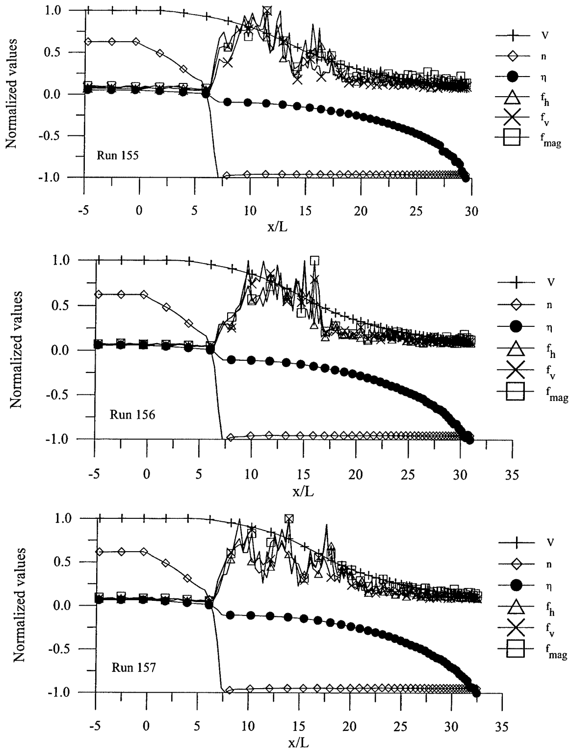
Figure 3.85 Development of RMS propeller horizontal and vertical forces and RMS propeller force magnitude during unsteady crashback maneuver simulation (extended data stream)
