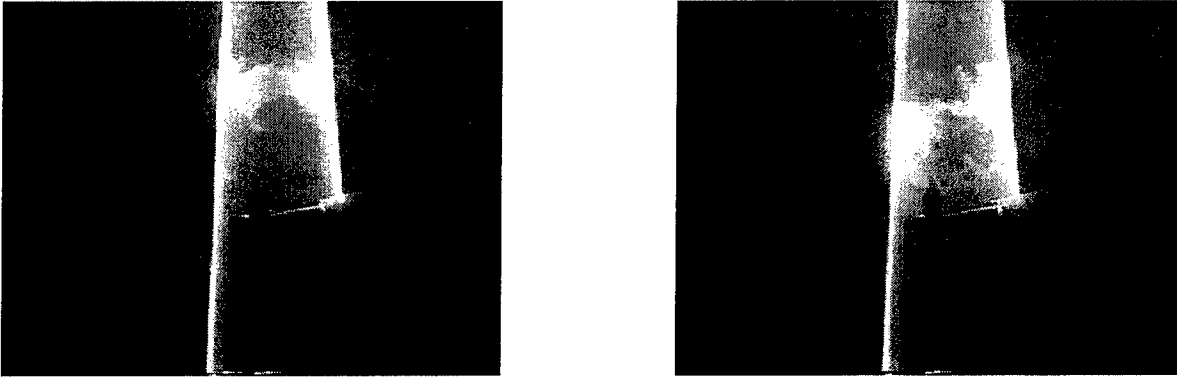
Figure 4.44 Flow visualization images at V = 2.5 kts, n = 600 RPM, \eta = -2.17
