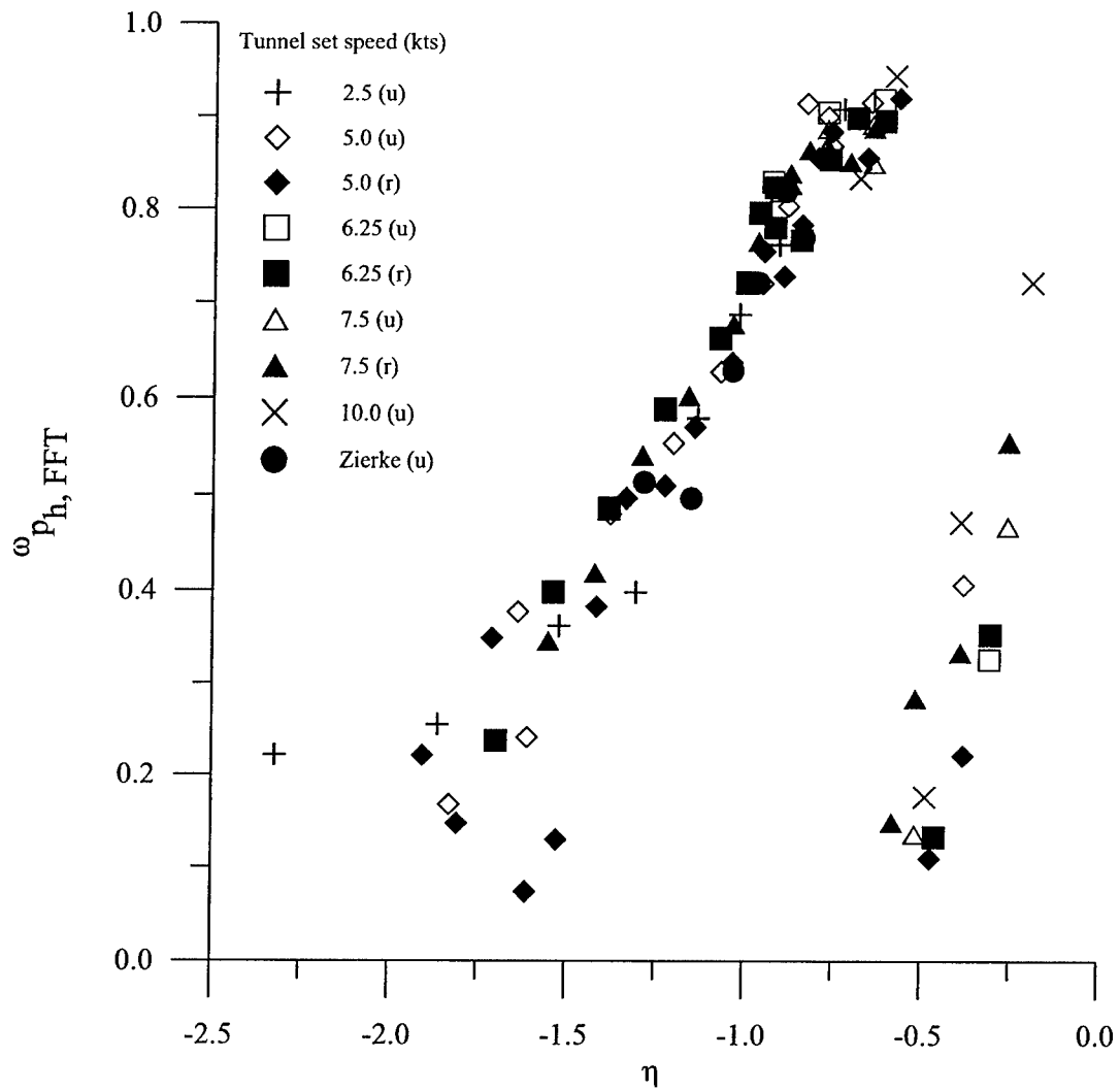
Figure 3.57 Dimensionless frequency of peak propeller horizontal force amplitude (“u” - model restraining strut off, “r” - model restraining strut on)
