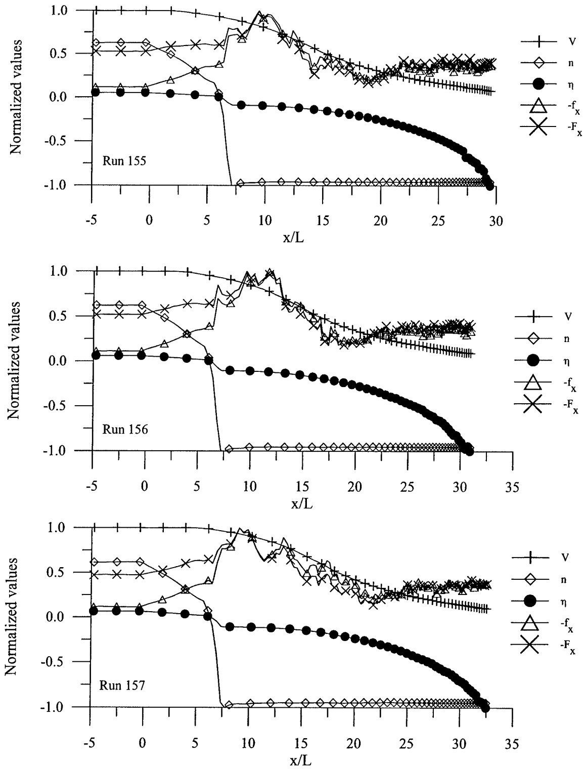
Figure 3.82 Development of RMS body axial force and moment during unsteady crashback maneuver simulation (extended data stream)
