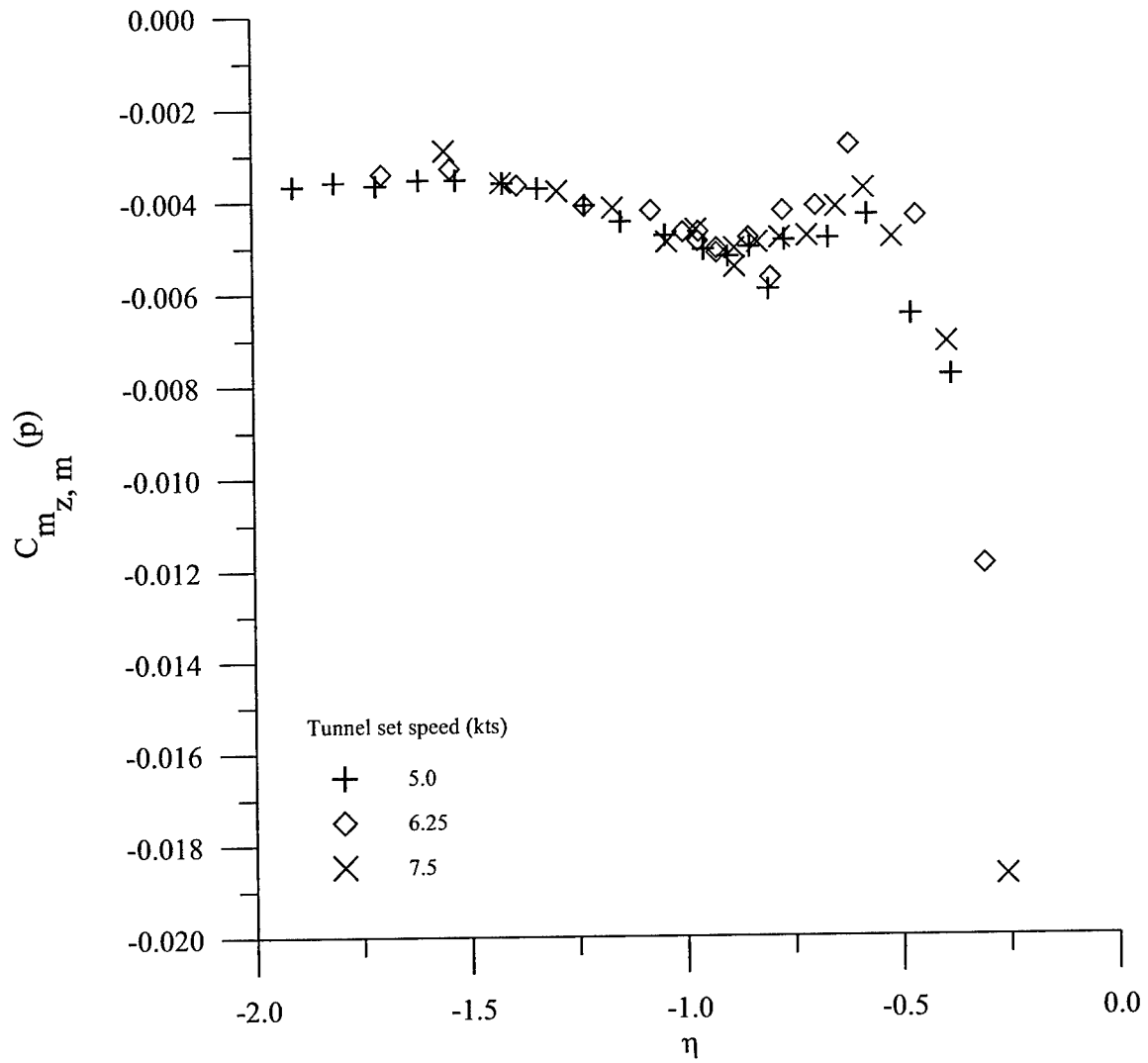
Figure 3.48 Coefficient of mean propeller z moment ("p" - propulsive scaling; all data with model restraining strut on)
