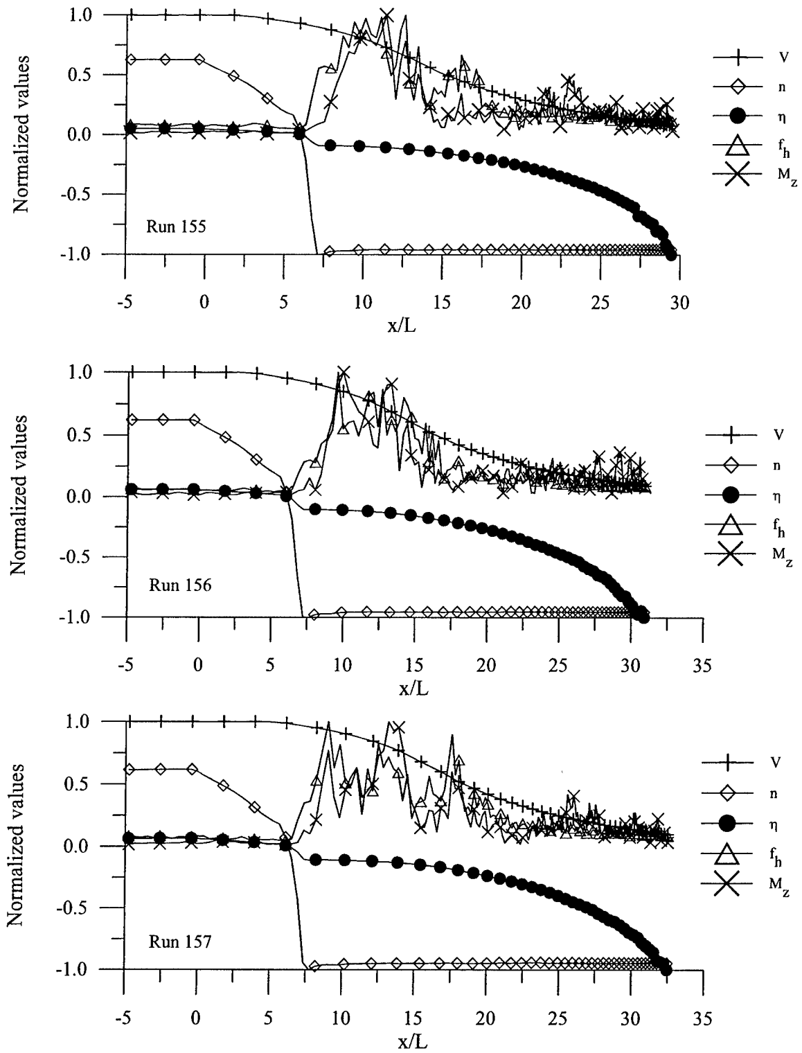
Figure 3.86 Development of RMS propeller horizontal force and RMS body yawing moment during unsteady crashback maneuver simulation (extended data stream)
