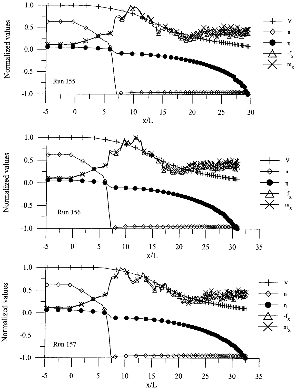
Figure 3.81 Development of RMS propeller axial force and moment during unsteady crashback maneuver simulation (extended data stream)
