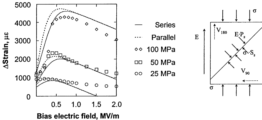
Figure 3: Analytical and experimental data for total compressive strain as a function of bias electric field.
