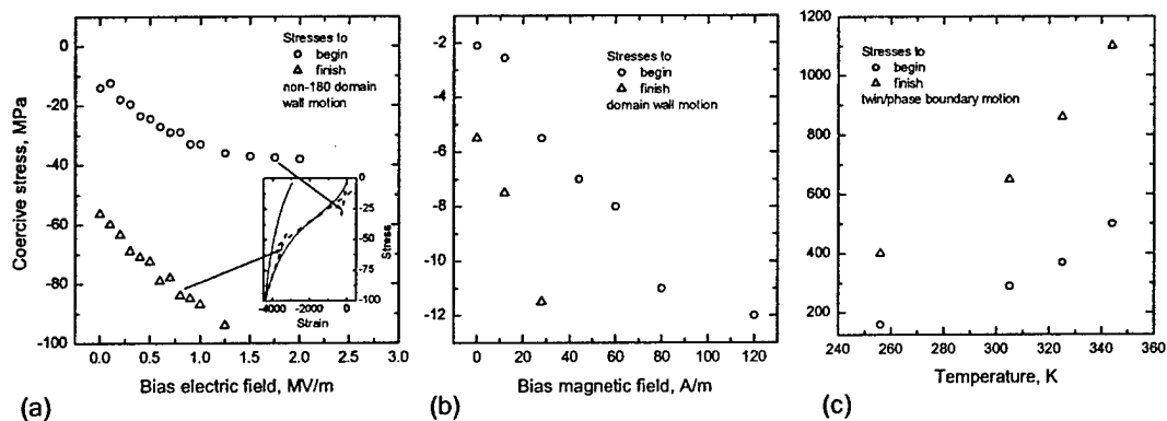
Figure 2: Critical stresses to begin and end strain jump in (a) piezoelectric; (b) magnetostrictive; (c) shape memory materials.
