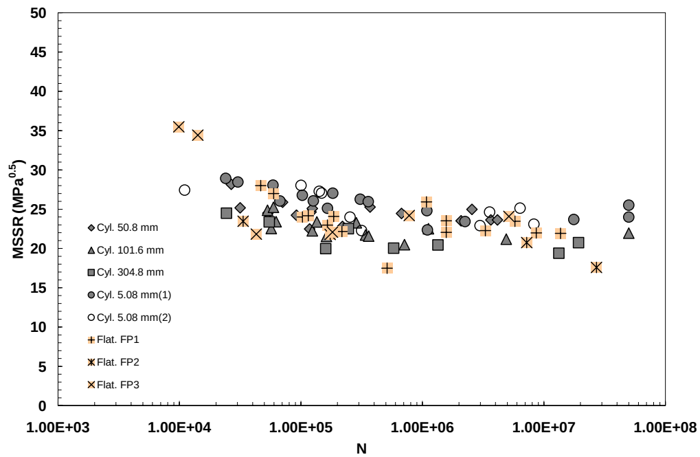
Figure 52. MSSR Parameter versus Fretting Fatigue Life Using Contact Surface Stresses
