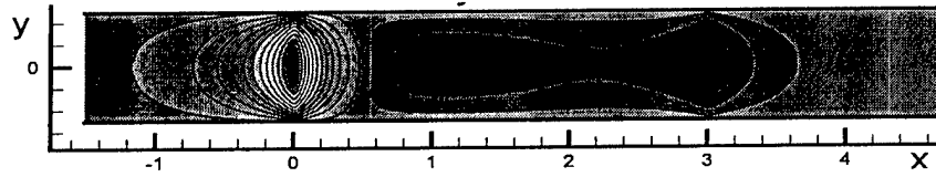
Figure 22. B_y Field., With \vec{V} \cdot \vec{B} = 0 control
