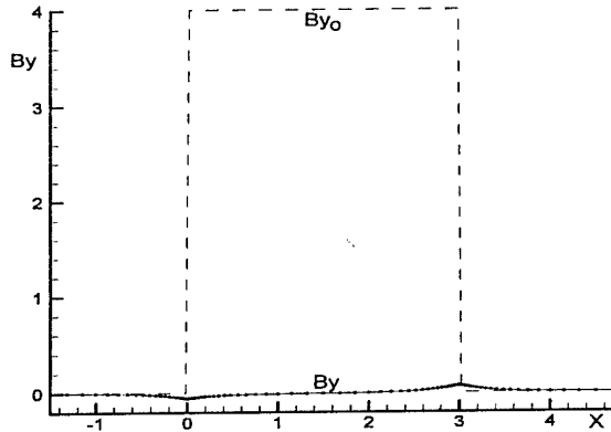
Figure 13. Solution for B_y along centerline.
